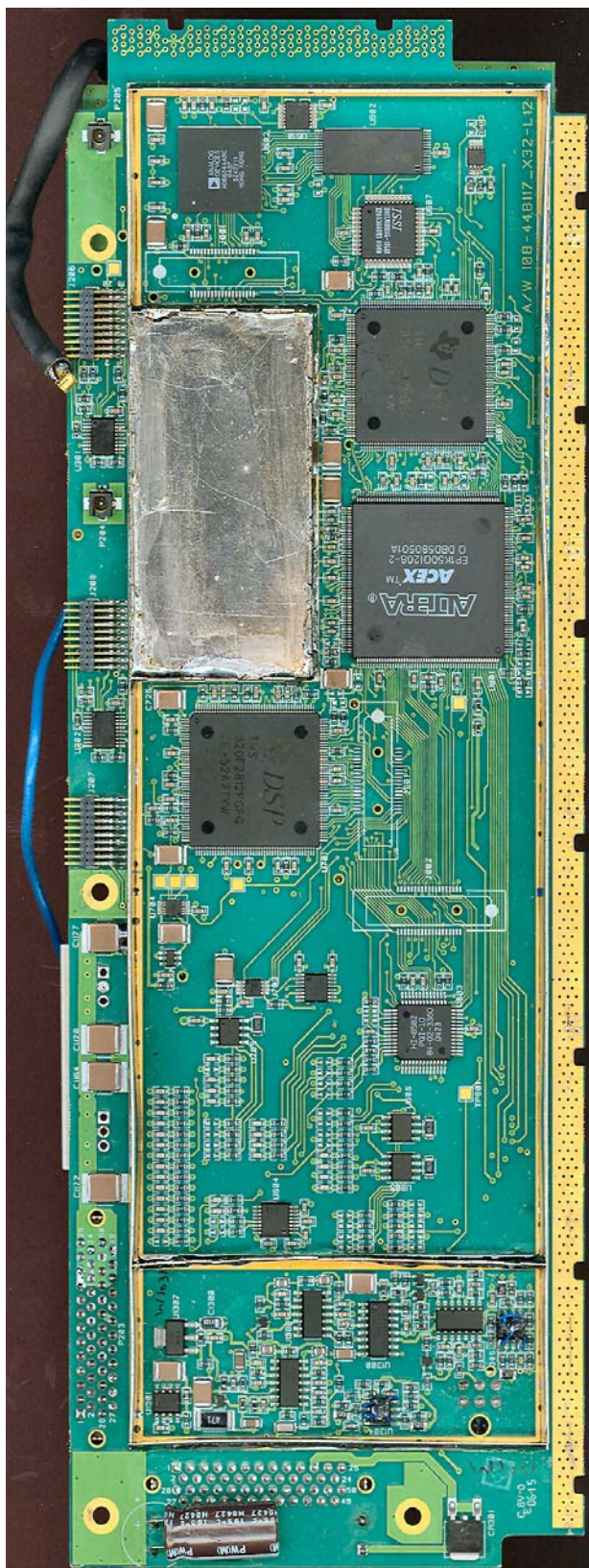
Bottom Side without Shield
