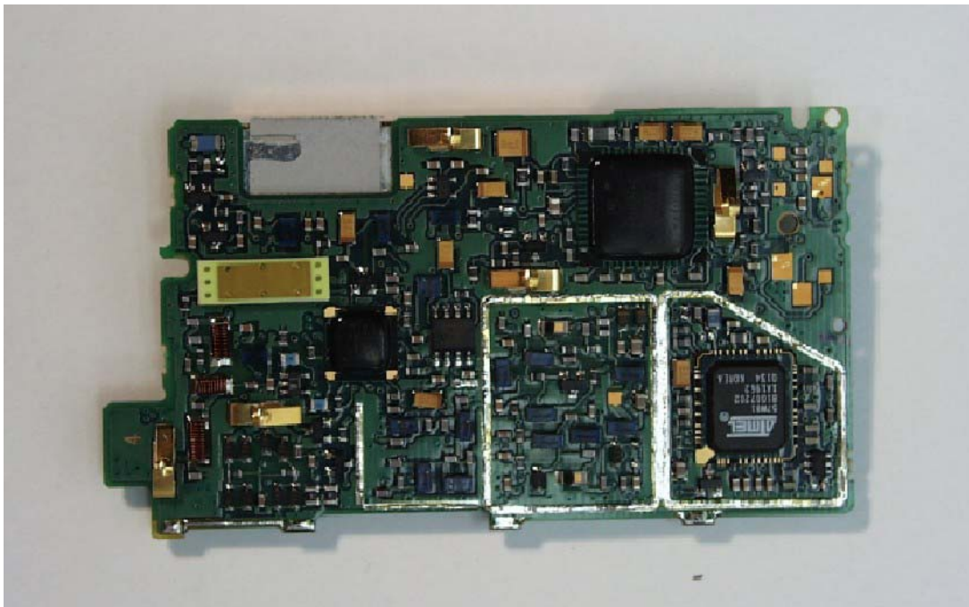
UHF-2 RF Board without Shields - Bottom View
