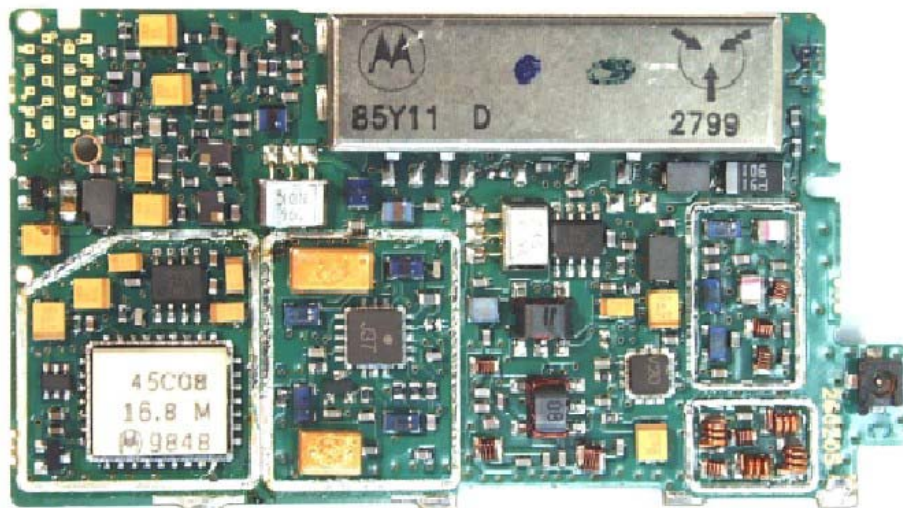
UHF-2 RF Board without Shields - Top View
