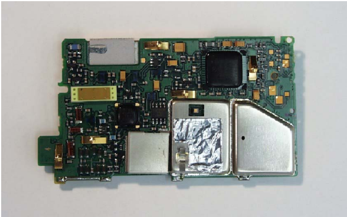
UHF-2 RF Board with Shields - Bottom View
