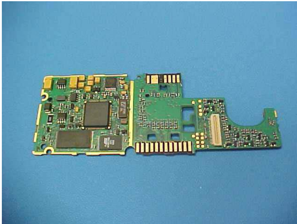
UHF-2 Controller Board - Top View
