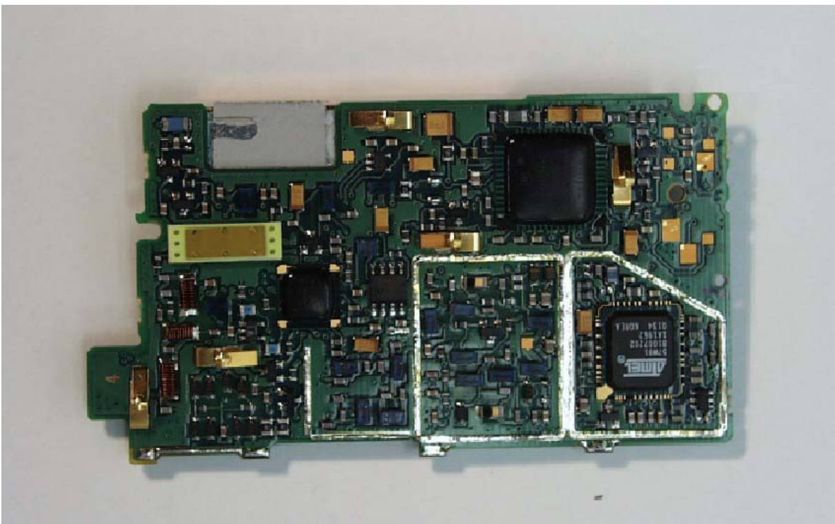
UHF-1 RF Board without Shields - Bottom View
