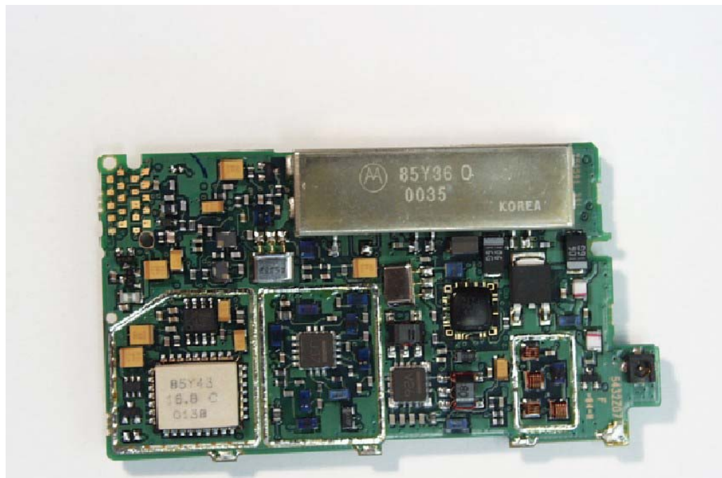
UHF-1 RF Board with Shields - Top View
