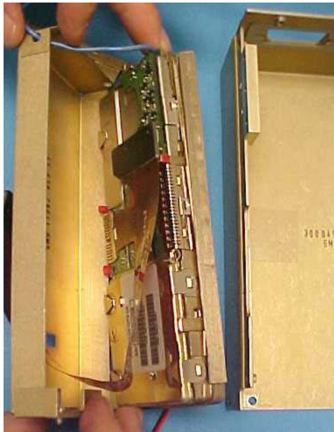
Step 6: ITM Cover removed reveals the ITM module inside with ribbon cable and blue RF cable.
