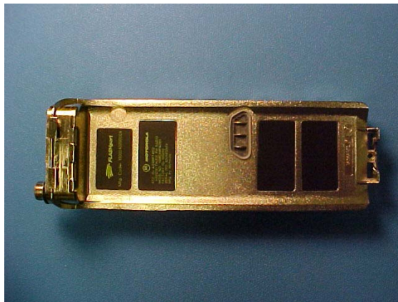
800 MHz Integrated Transceiver Module - Bottom View
