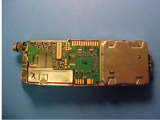
800 MHz Integrated Transceiver Module - Top View
