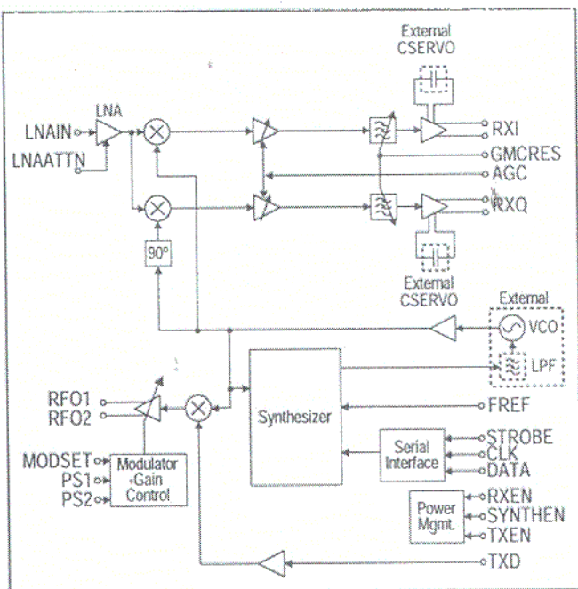
CR-201 RF Block Diagram
