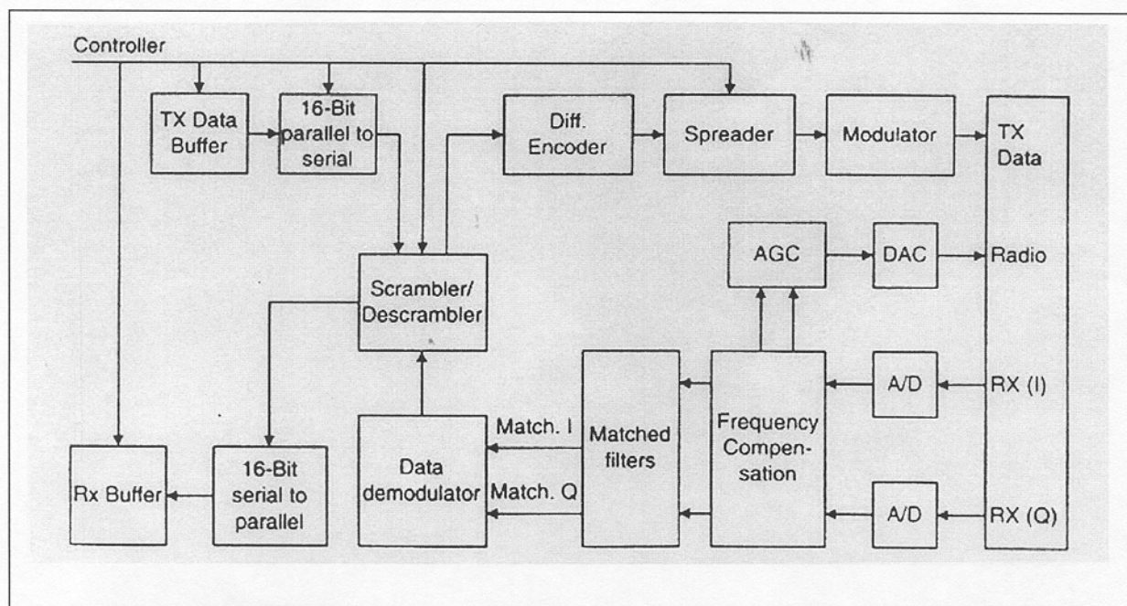
DSST Spread Spectrum Engine Block Diagram
