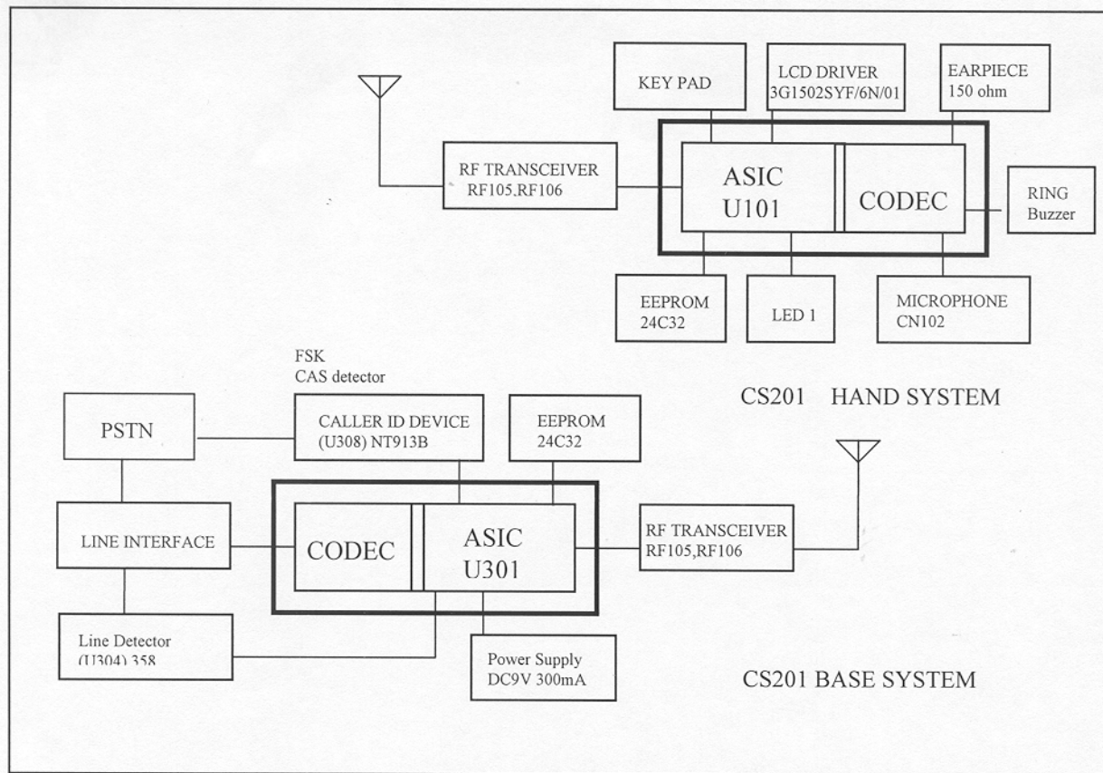
CS201 System Architecture
