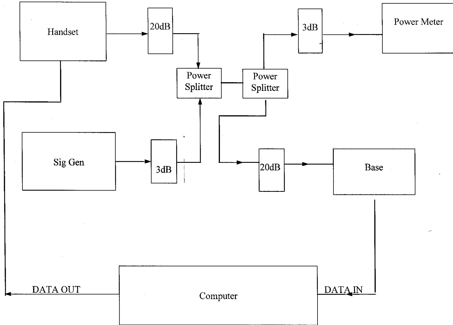
Jamming Test Setup for base unit
