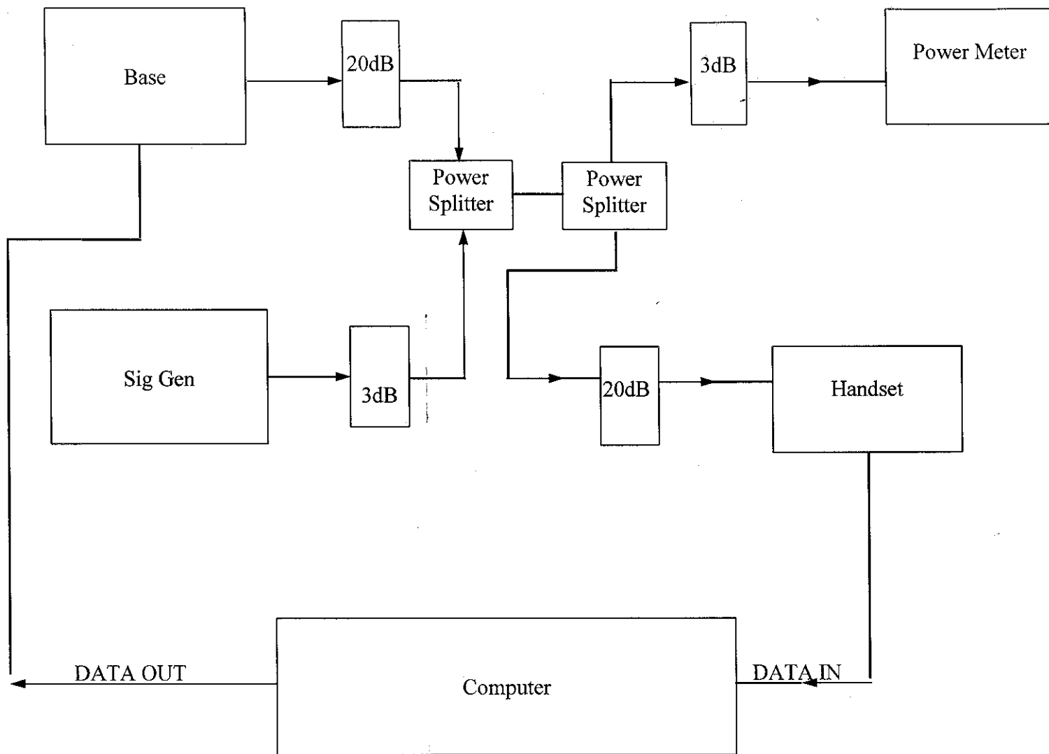
Jamming Test Setup for handset unit
