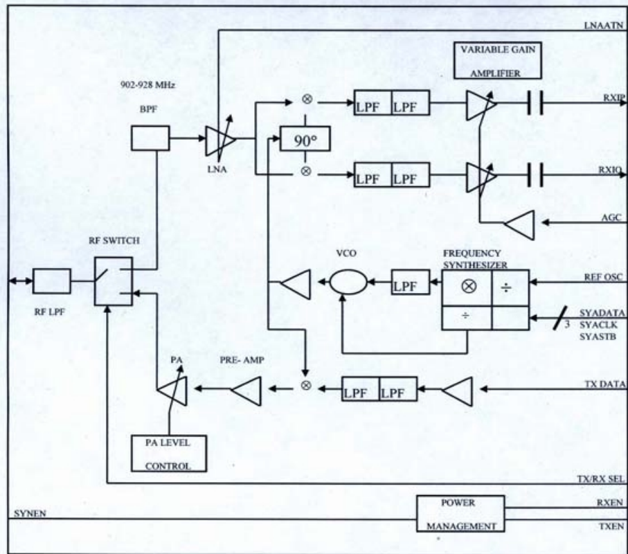
RF Block Diagram
