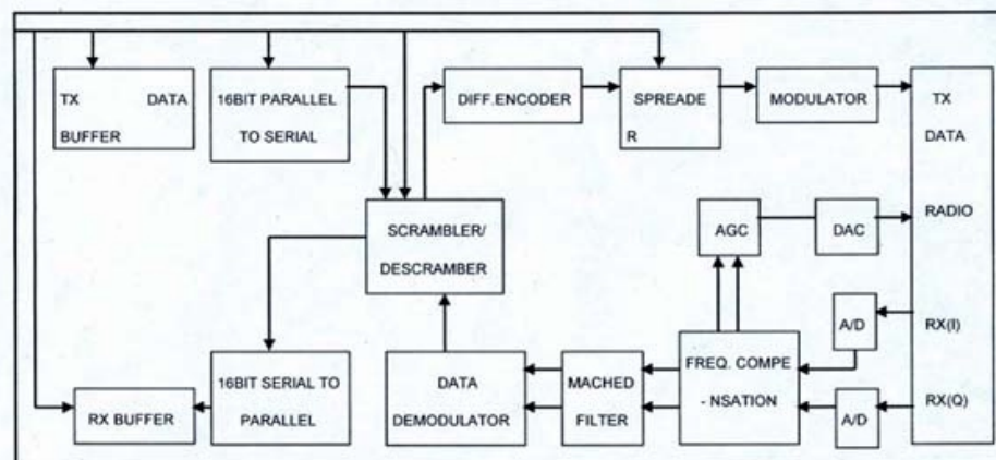
DCT Spread Spectrum Engine Block Diagram
