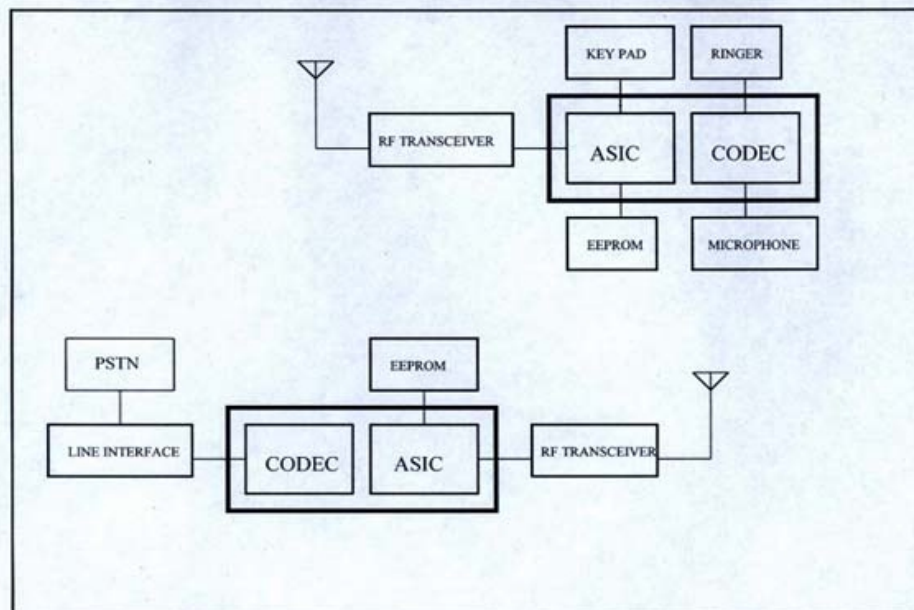
IS - 903 System Architecture
