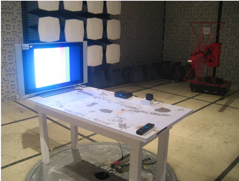
TEST SETUP OF RADIATED EMISSION (HDMI AND AVOUT MODEL)
