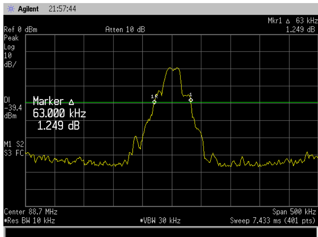
88.7MHZ bandwidth test plot
