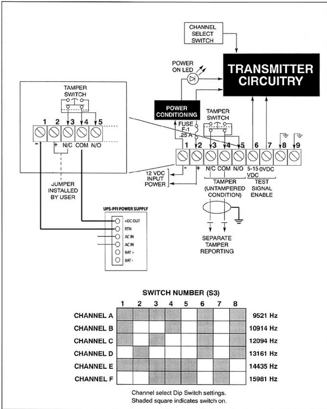
Figure 11: Transmitter Wiring
