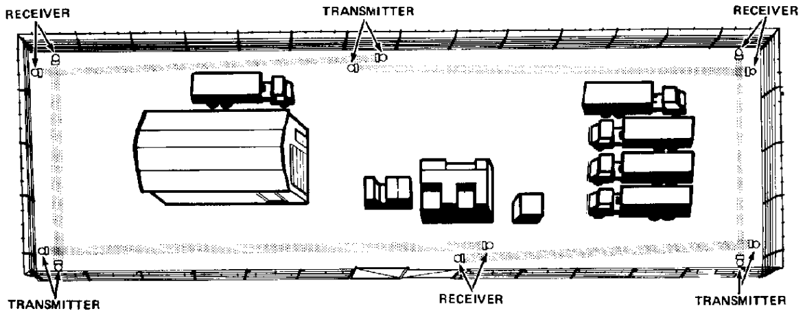
Figure 6: Perimeter Layout
