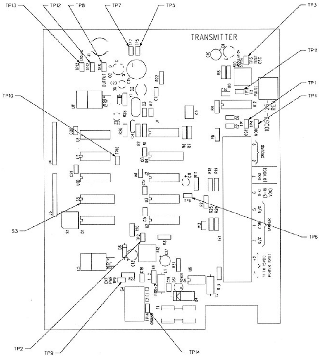
Figure 16: Transmitter Circuit Board Component Location
