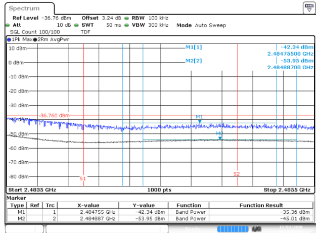
Date: 3 DEC 2020 16:17:55 BE-R-HIGH-2MHz, SISO-A, 802.11ax20-HE0, Ch13
