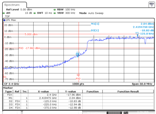
Date: 3 DEC 2020 16:22:42 BE-NR, SISO-A, 802.11ax40-HE0, Ch3
