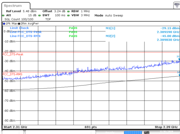
Date: 3 DEC 2020 16:22:33 BE-R-LOW, SISO-A, 802.11ax40-HE0, Ch3
