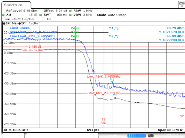
Date: 3 DEC 2020 16:17:46 BE-R-HIGH, SISO-A, 802.11ax20-HE0, Ch13
