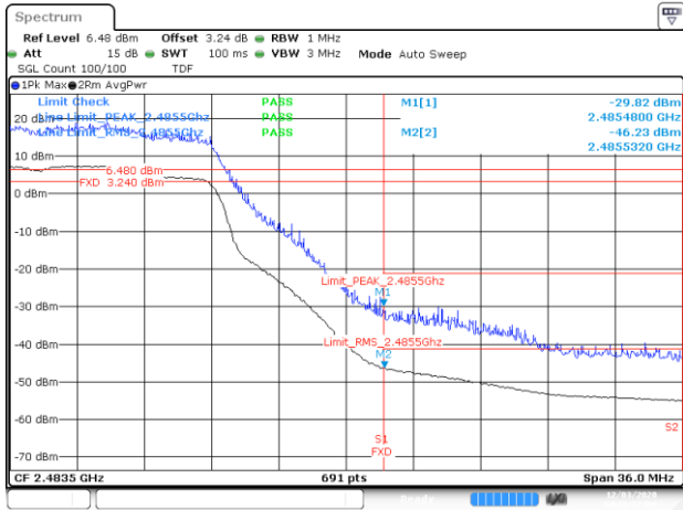
Date: 3 DEC 2020 16:16:37 BE-R-HIGH, SISO-A, 802.11ax20-HE0, Ch12
