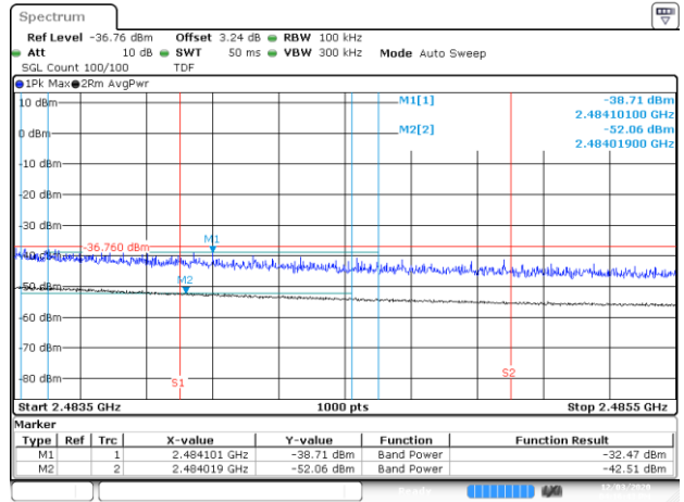
Date: 3 DEC 2020 16:16:43 BE-R-HIGH-2MHz, SISO-A, 802.11ax20-HE0, Ch12
