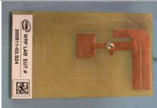
Main Antenna
