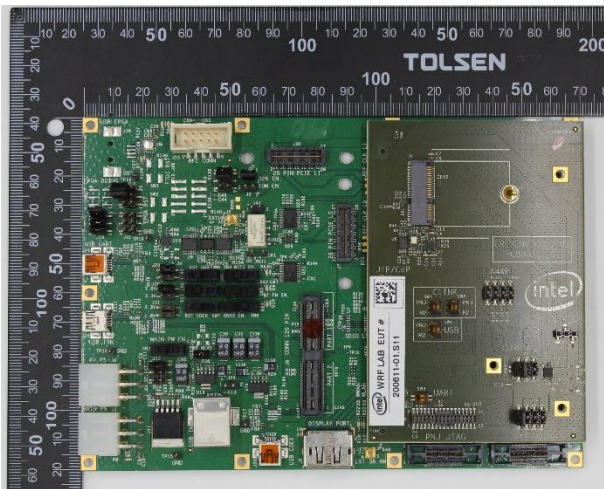
Extender board
