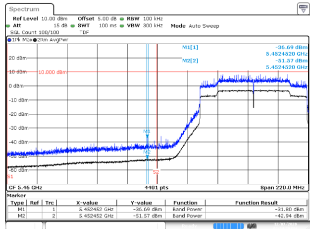
BE-R-LOW, SISO-A, 802.11ax80-HE0, Ch106
