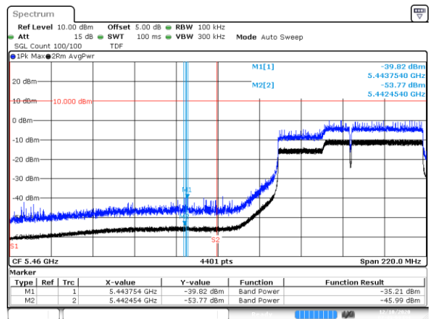
BE-R-LOW, MIMO-B, 802.11ac160-VHT0, Ch114
