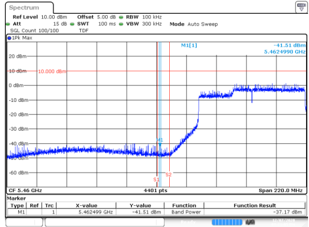
Date: 7 DEC 2020 15:31:05 BE-NR-LOW, SISO-A, 802.11ax160-HE0, Ch114
