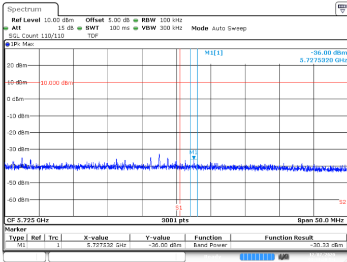
Date: 7 DEC 2020 15:31:20 BE-NR-HIGH, SISO-A, 802.11ax160-HE0, Ch114
