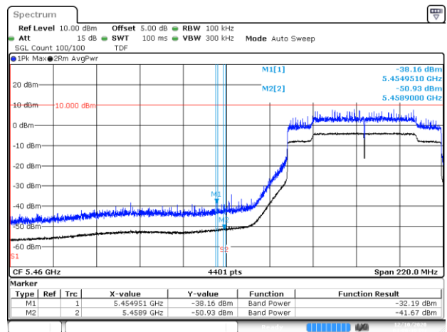
BE-R-LOW, SISO-B, 802.11ax80-HE0, Ch106
