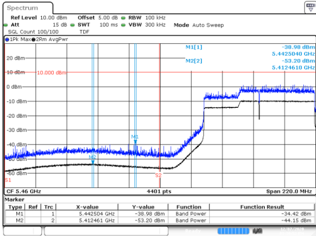
Date: 7 DEC 2020 15:30:53 BE-R-LOW, SISO-A, 802.11ax160-HE0, Ch114
