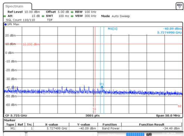
BE-NR-HIGH, MIMO-B, 802.11ac160-VHT0, Ch114
