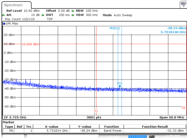
BE-NR-HIGH, MIMO-A, 802.11ac80-VHT0, Ch122
