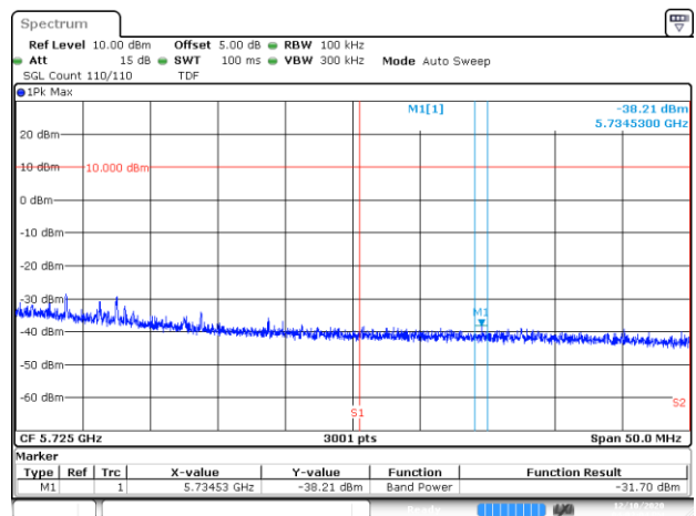
BE-NR-HIGH, SISO-B, 802.11ax80-HE0, Ch122
