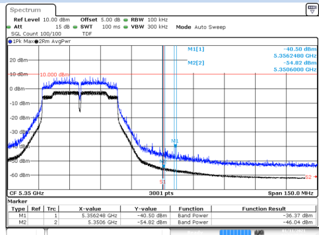
BE-R-HIGH, MIMO-B, 802.11n40-HT8, Ch62
