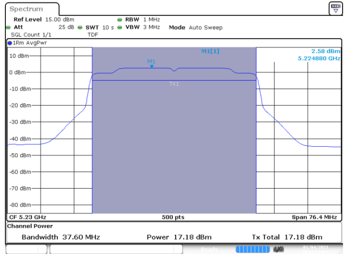
MIMO B-802.11ax-40MHz-Ch46-5230MHz-HE0
