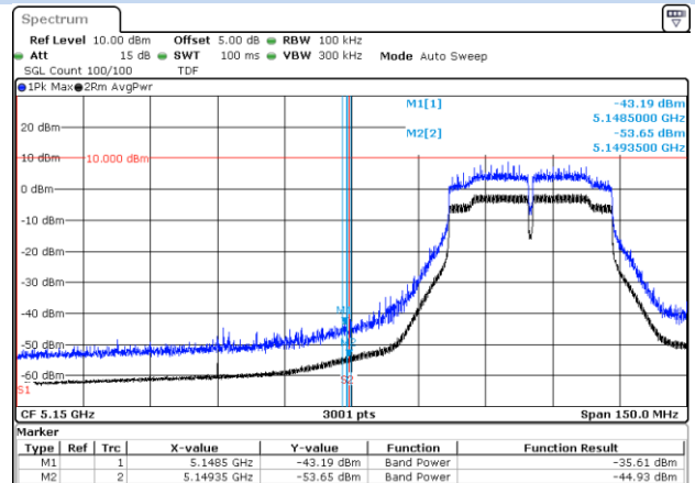
BE-R-LOW, MIMO-B, 802.11n40-HT8, Ch38
