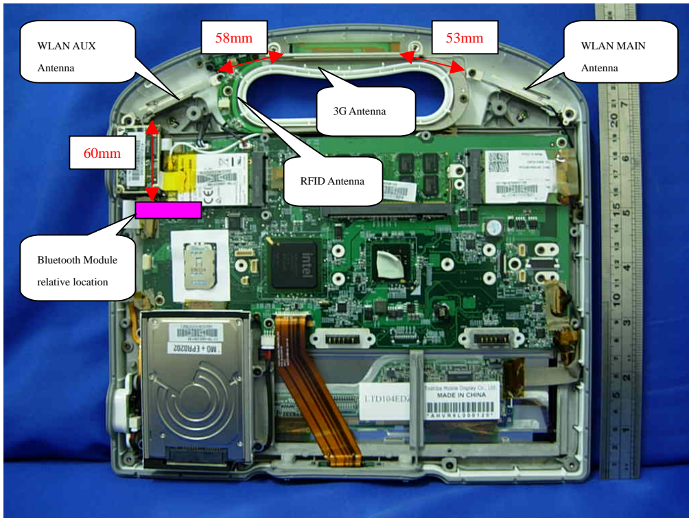
(38) EUT Photo
