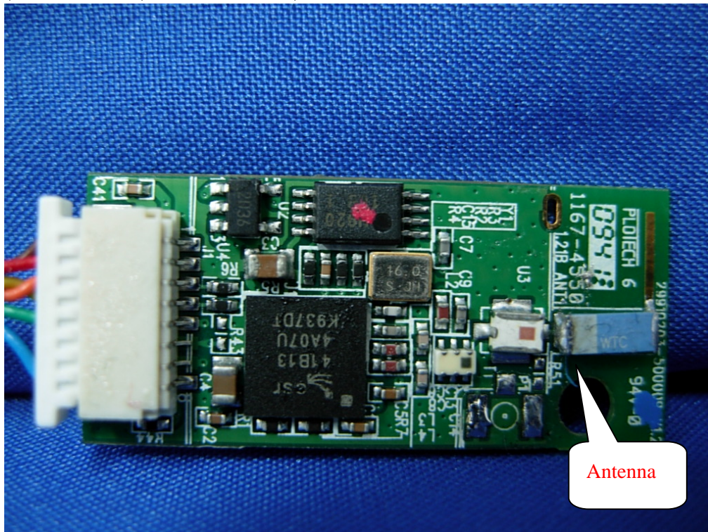
(13) EUT Photo - (Bluetooth Module)
