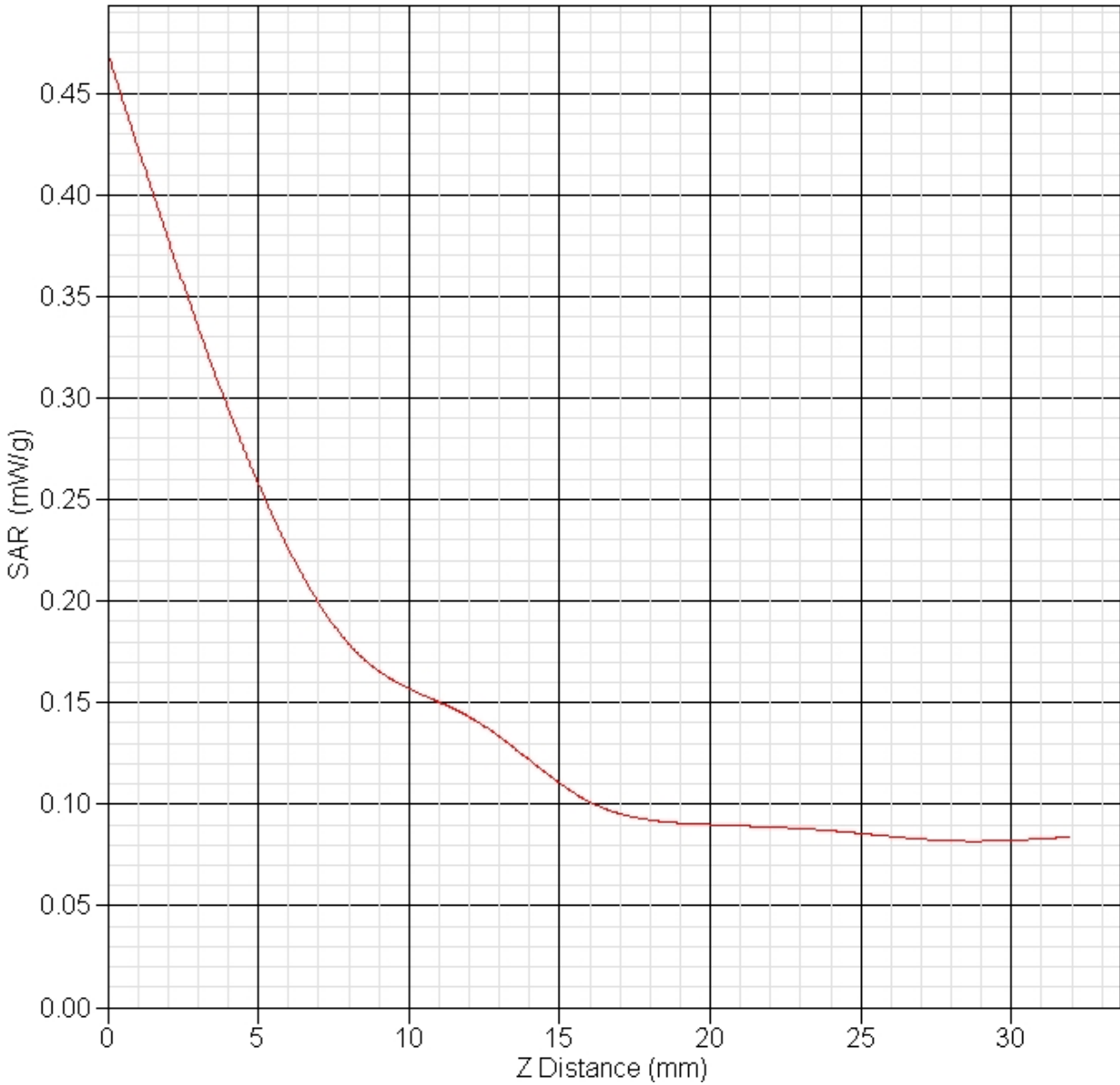
SAR-Z Axis at Hotspot x:0.01 y:-2.01
