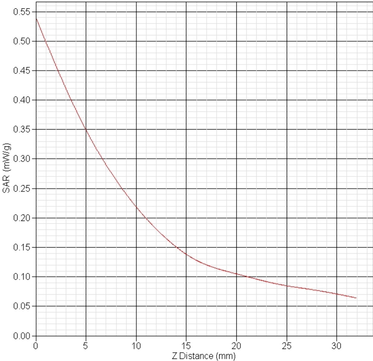
SAR-Z Axis at Hotspot x:0.07 y:-6.01
