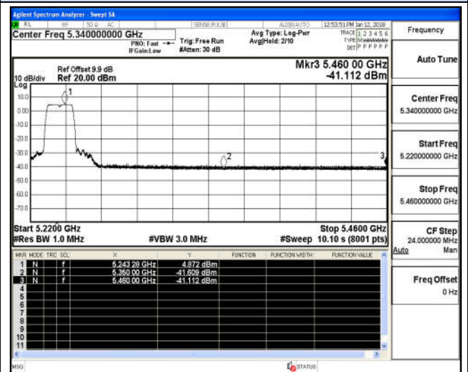
Channel 48 / 5240 MHz – Peak
