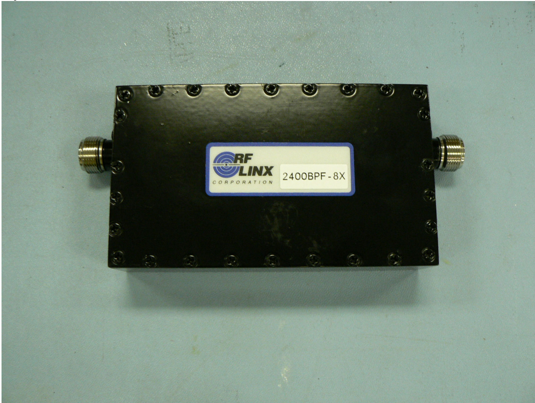
Cavity Filter
