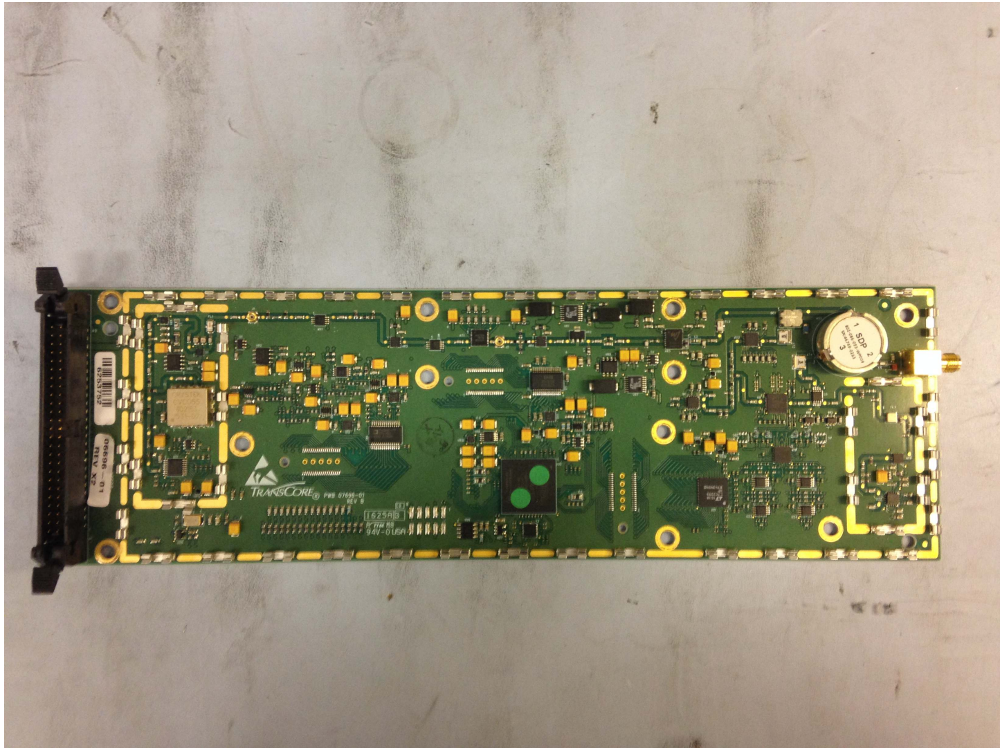
Figure 8 - Transceiver Front
