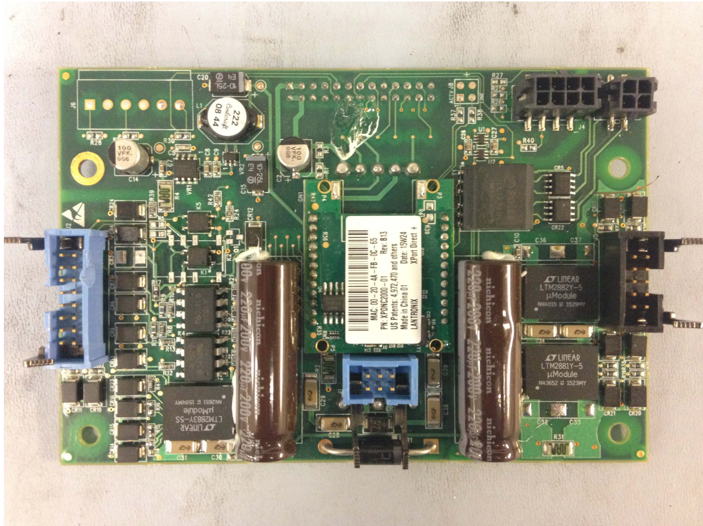
Figure 4 - IO Board Front
