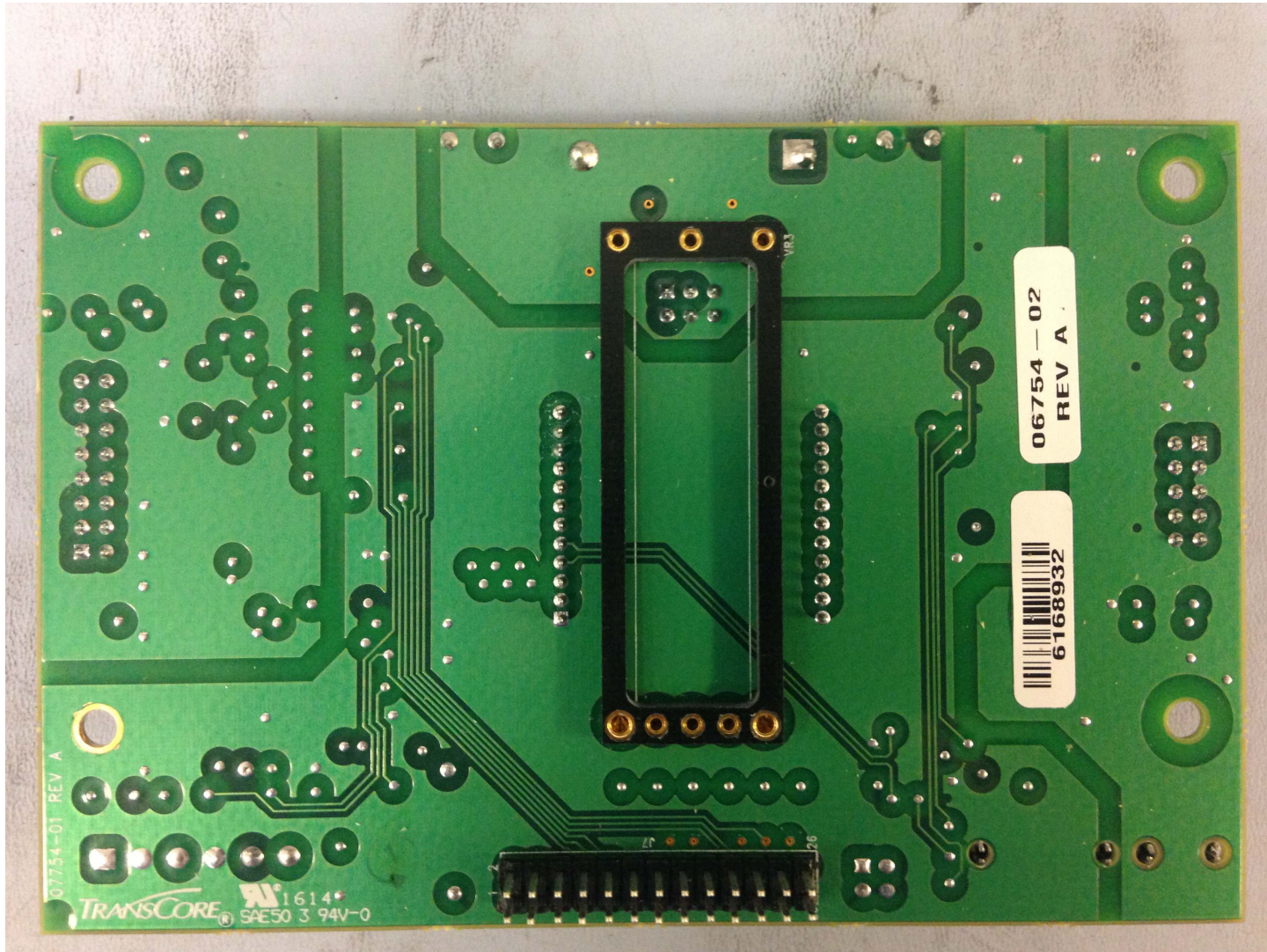
Figure 3 - IO Board Back
