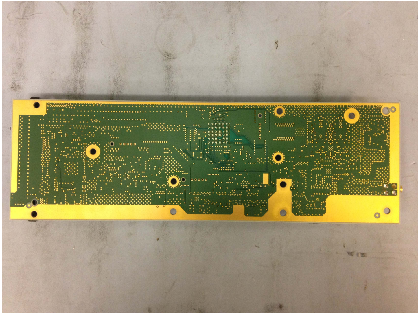
Figure 7 - Transceiver Back
