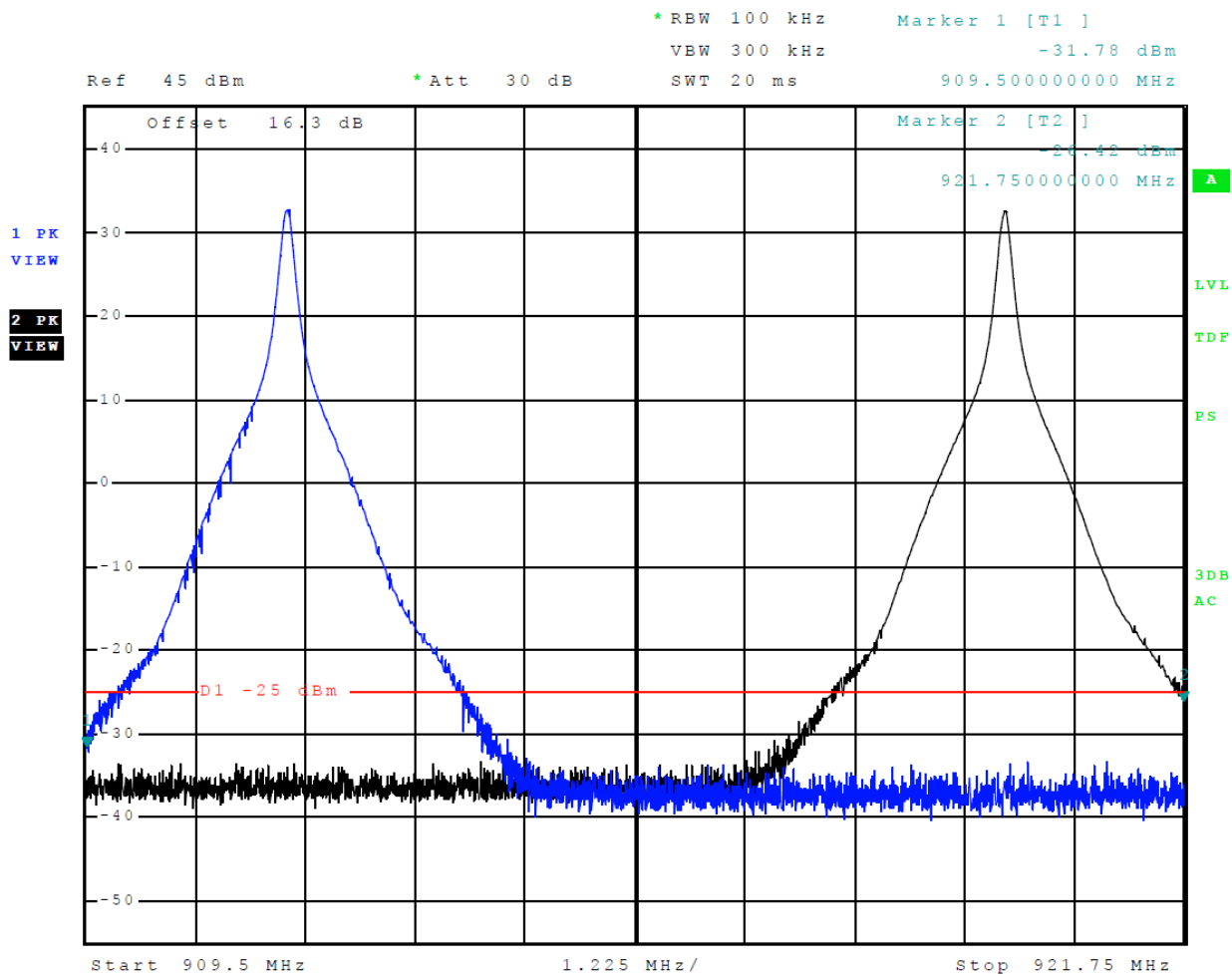
Figure 18 Emissions Mask eGo
