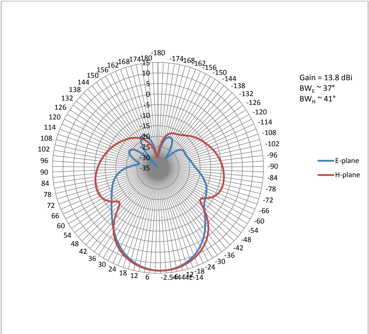
Figure 1. Gain of Antenna
