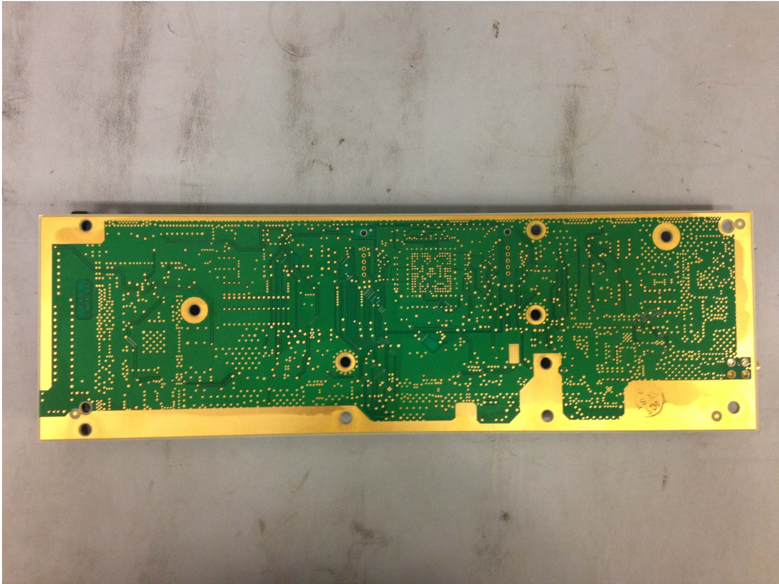
Figure 8 Radio 06588-02 Back
