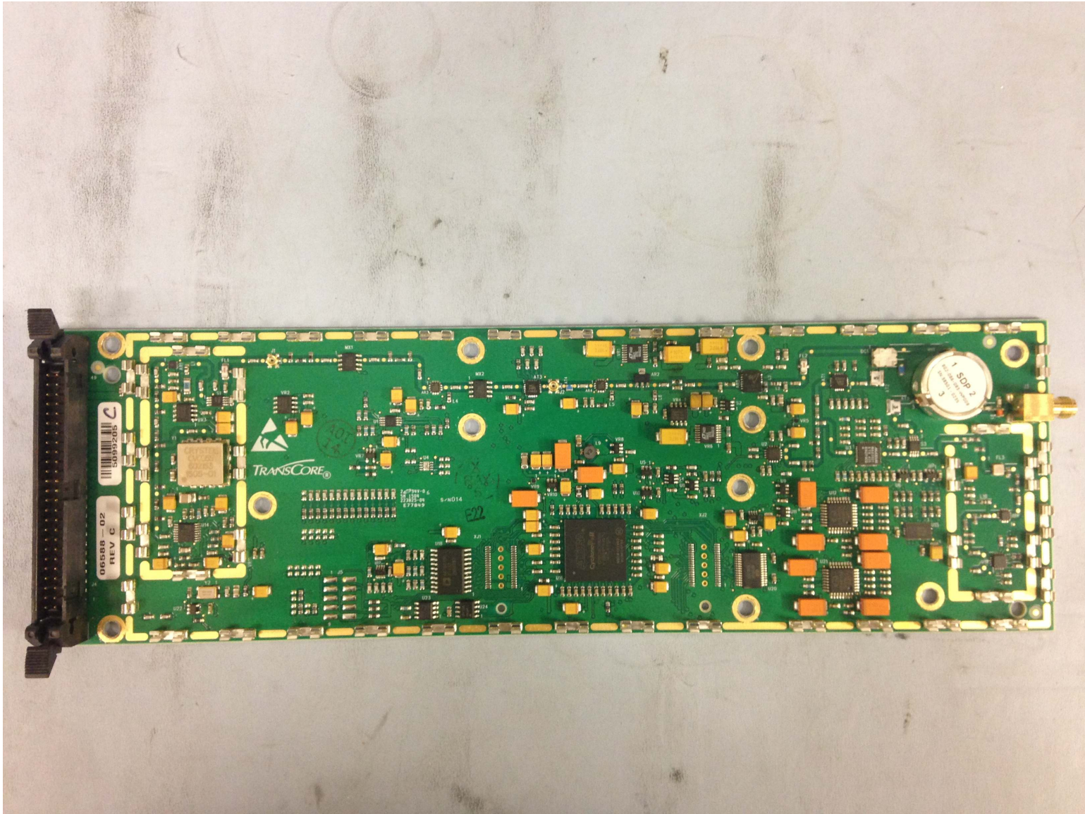
Figure 9 Radio 06588-02 Back
