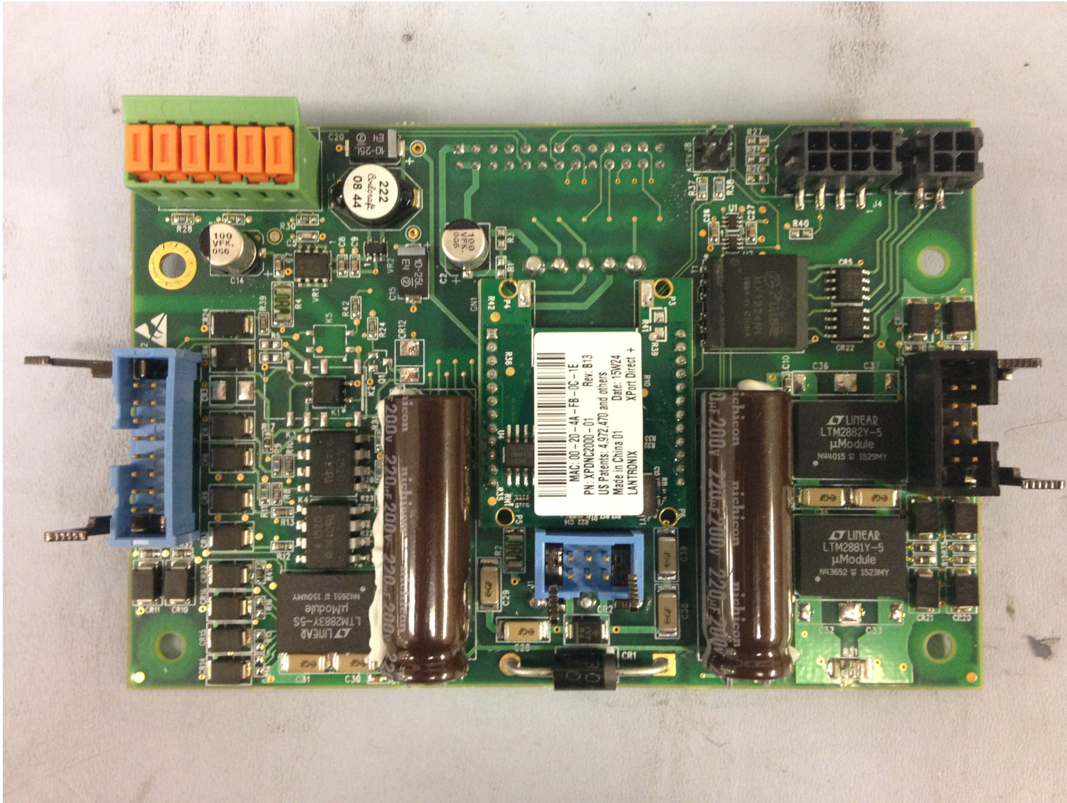
Figure 7 IO 06754-03 Top
