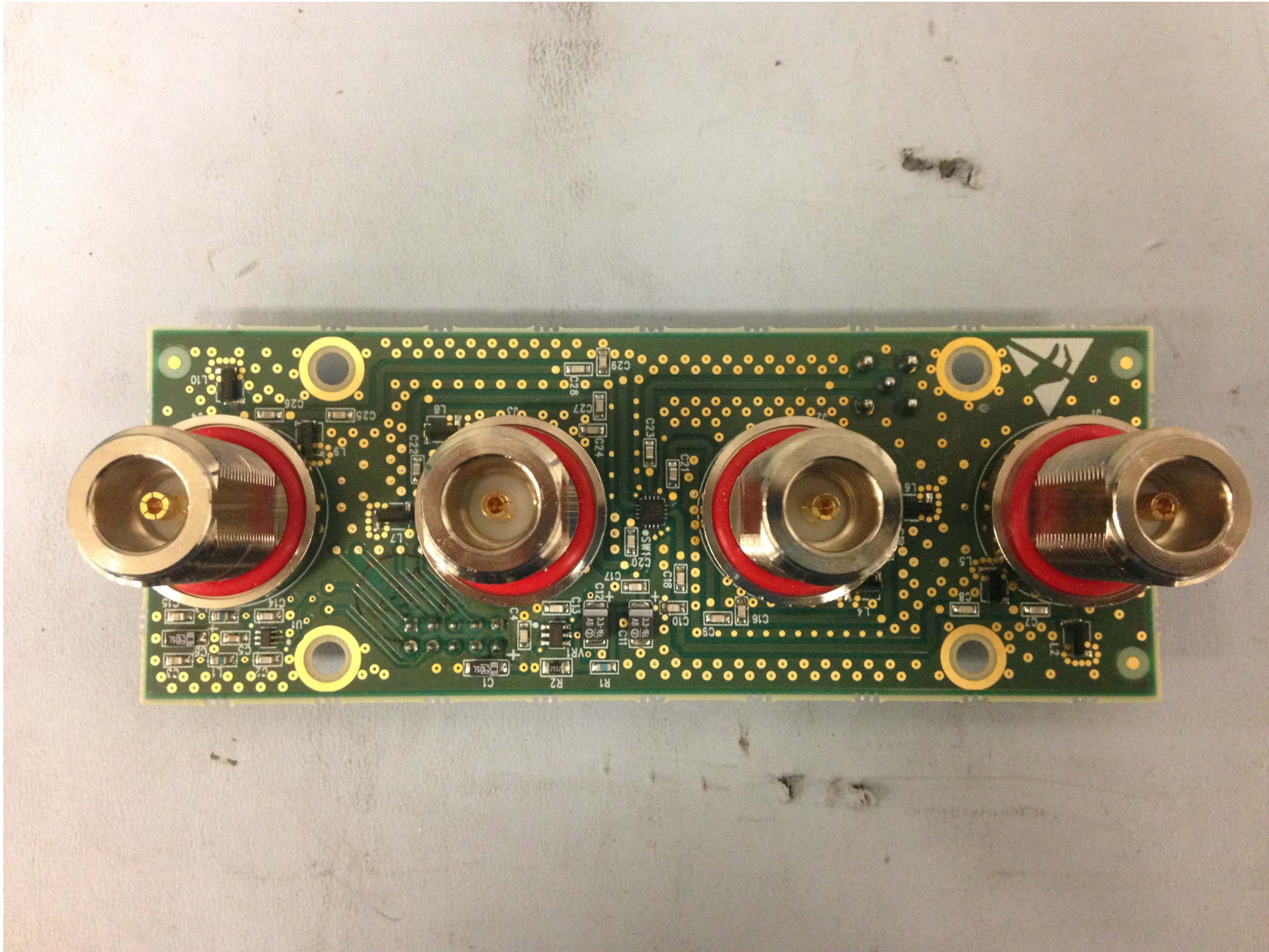
Figure 3 Antenna Mux 06569-01 Top
