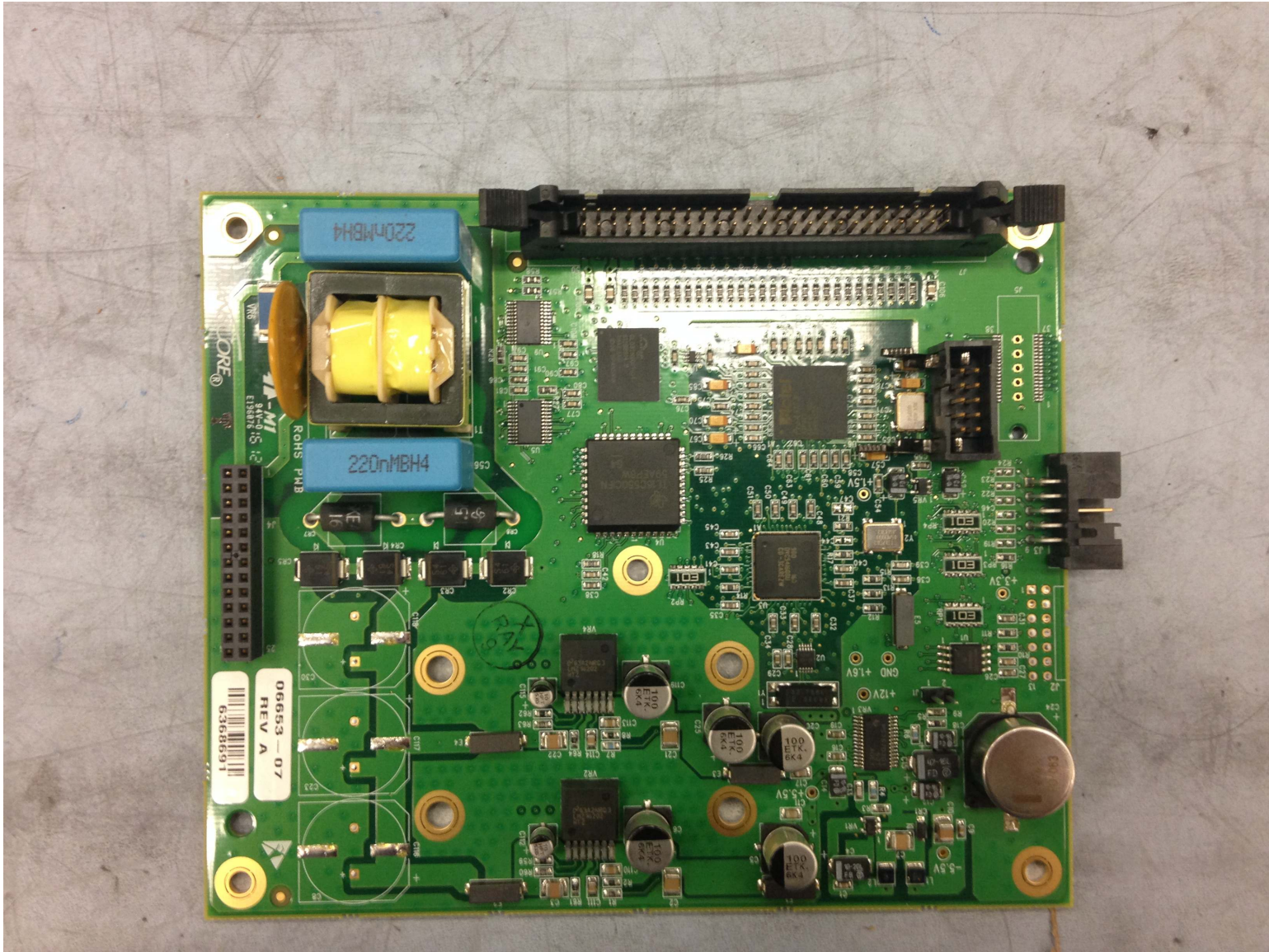
Figure 5DSP-PS 06653-07 Top
