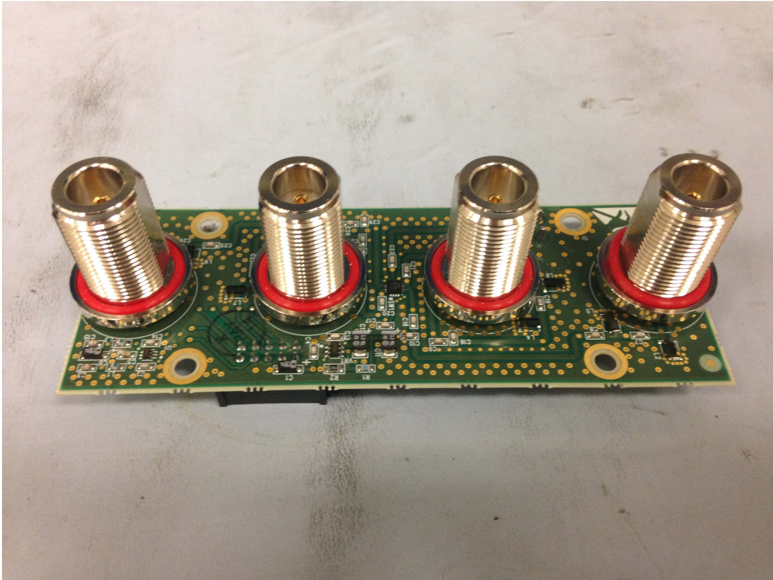
Figure 2 Antenna Mux 06569-01 Back
