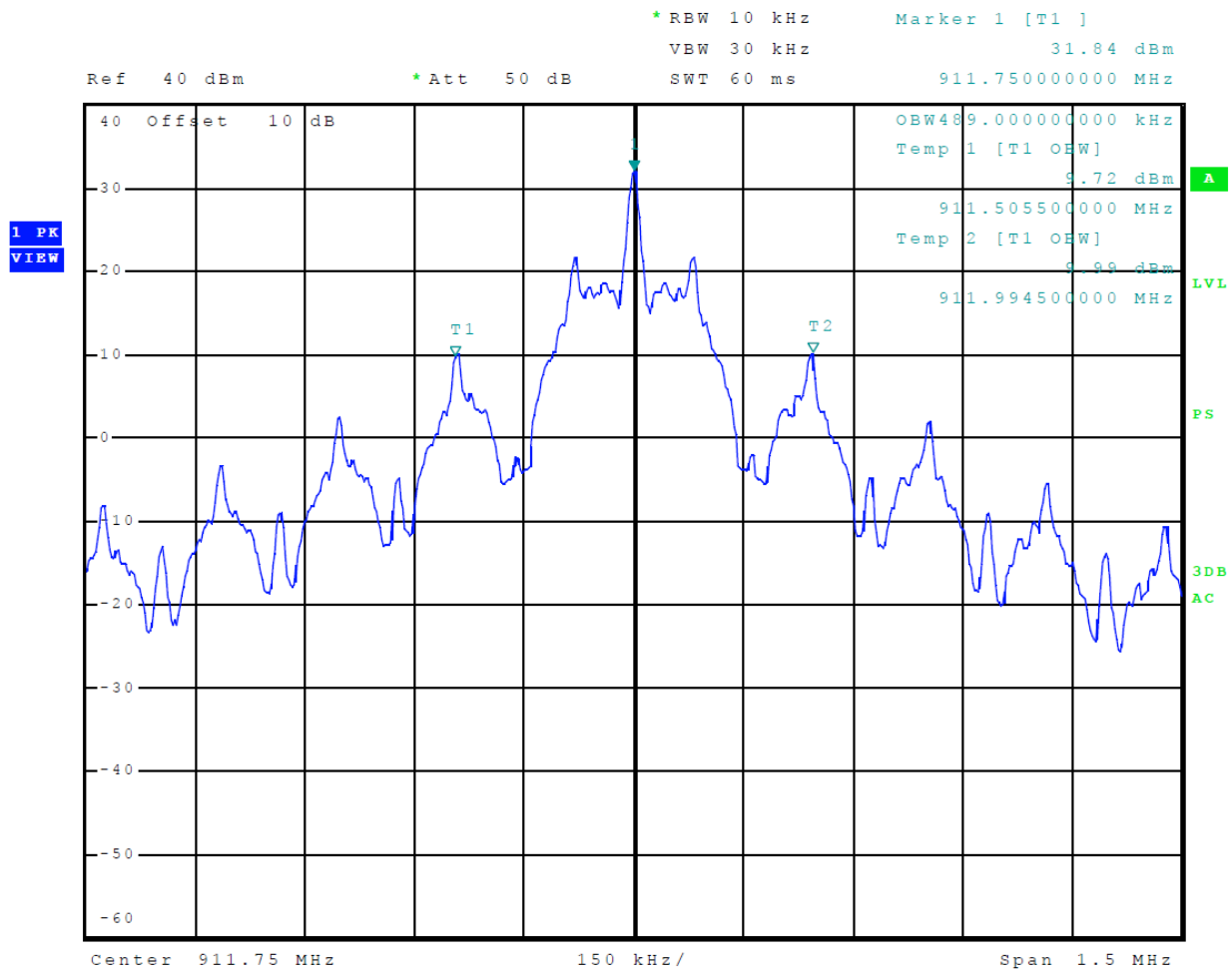
Figure 9 Occupied Bandwidth SeGo
