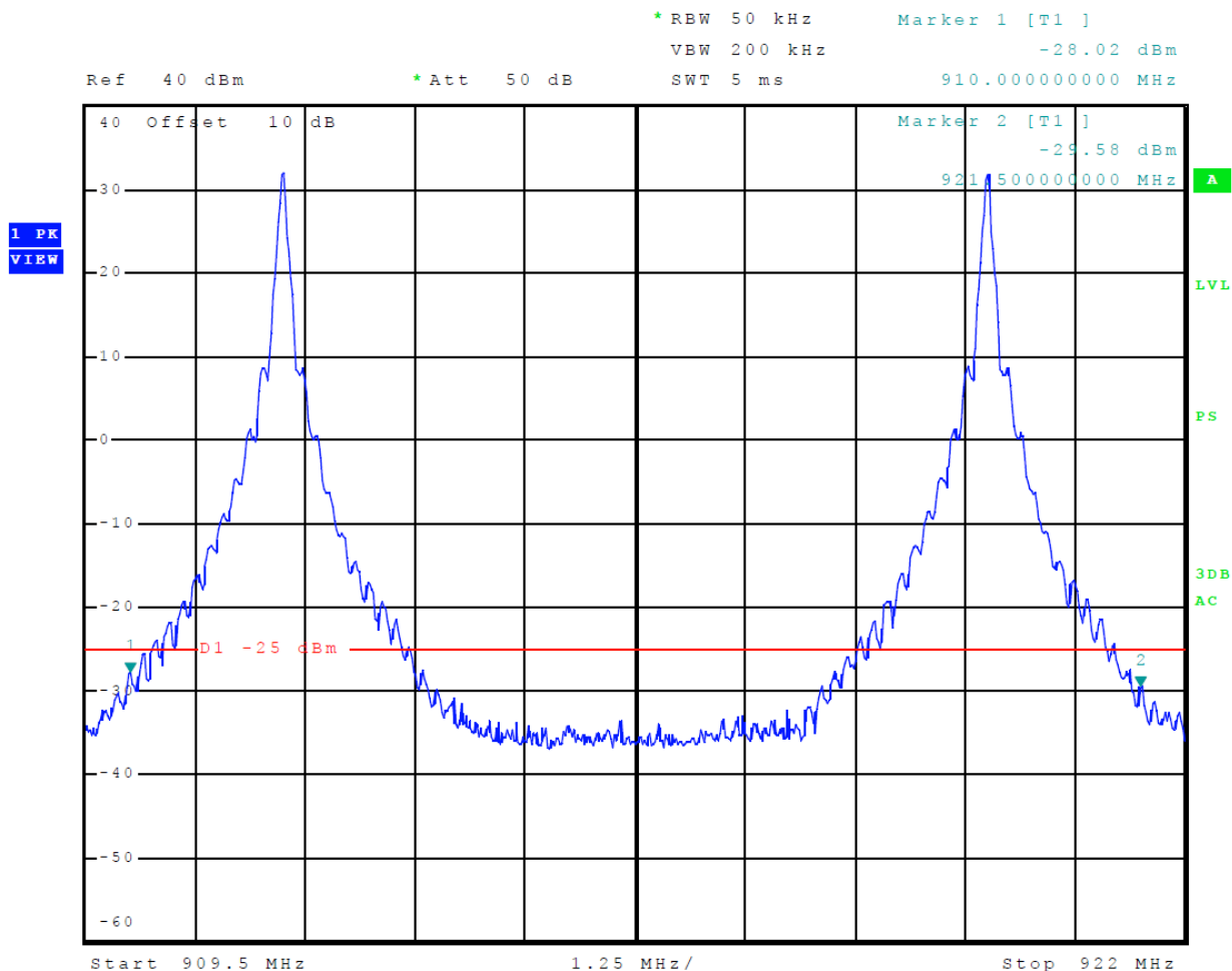
Figure 17 Emissions Mask EPC
