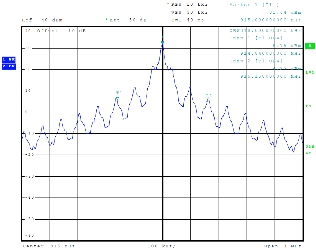
Figure 8 Occupied Bandwidth eGo
