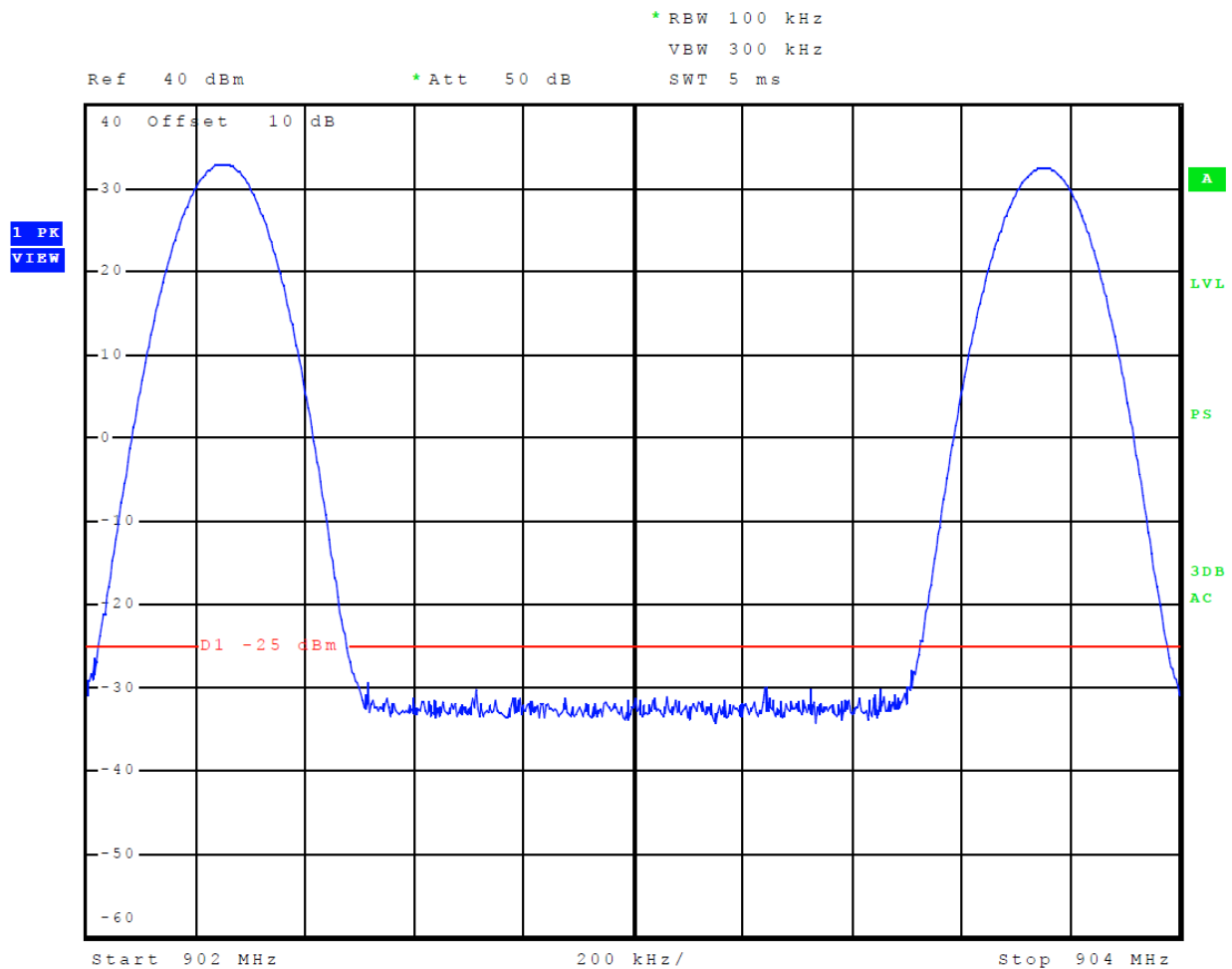
Figure 12 Emissions Mask ATA
