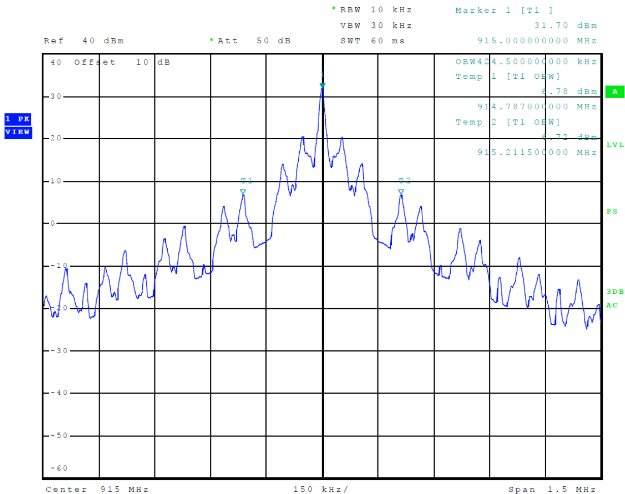
Figure 11 Occupied Bandwidth EPC
