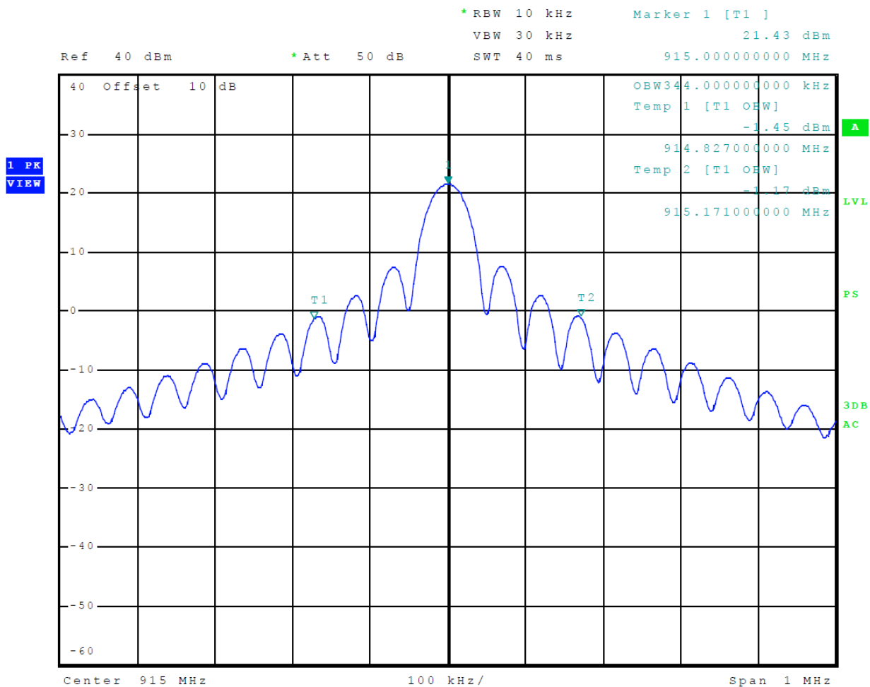
Figure 10 Occupied Bandwidth IAG
