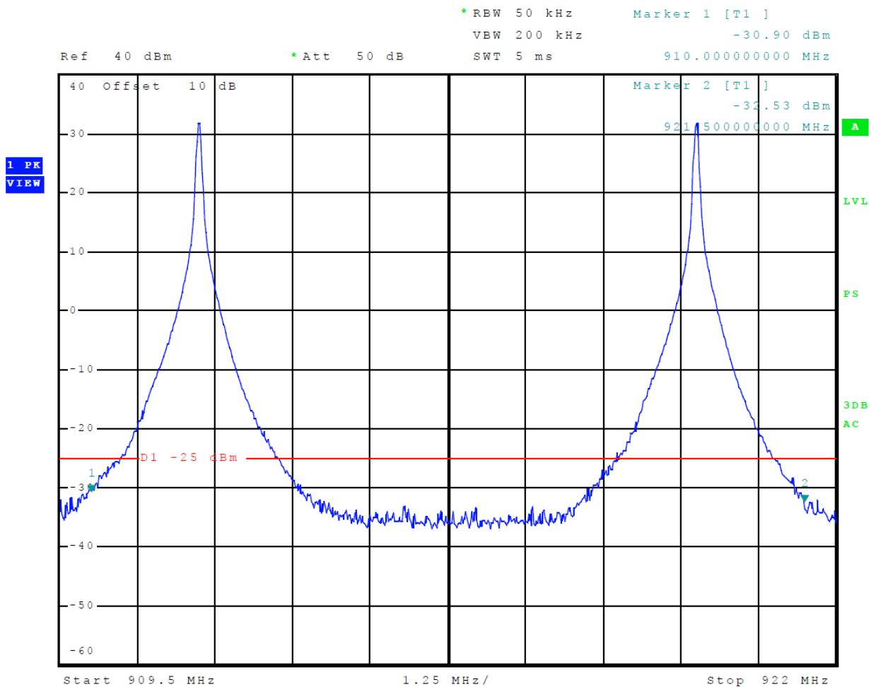
Figure 14 Emissions Mask eGo
