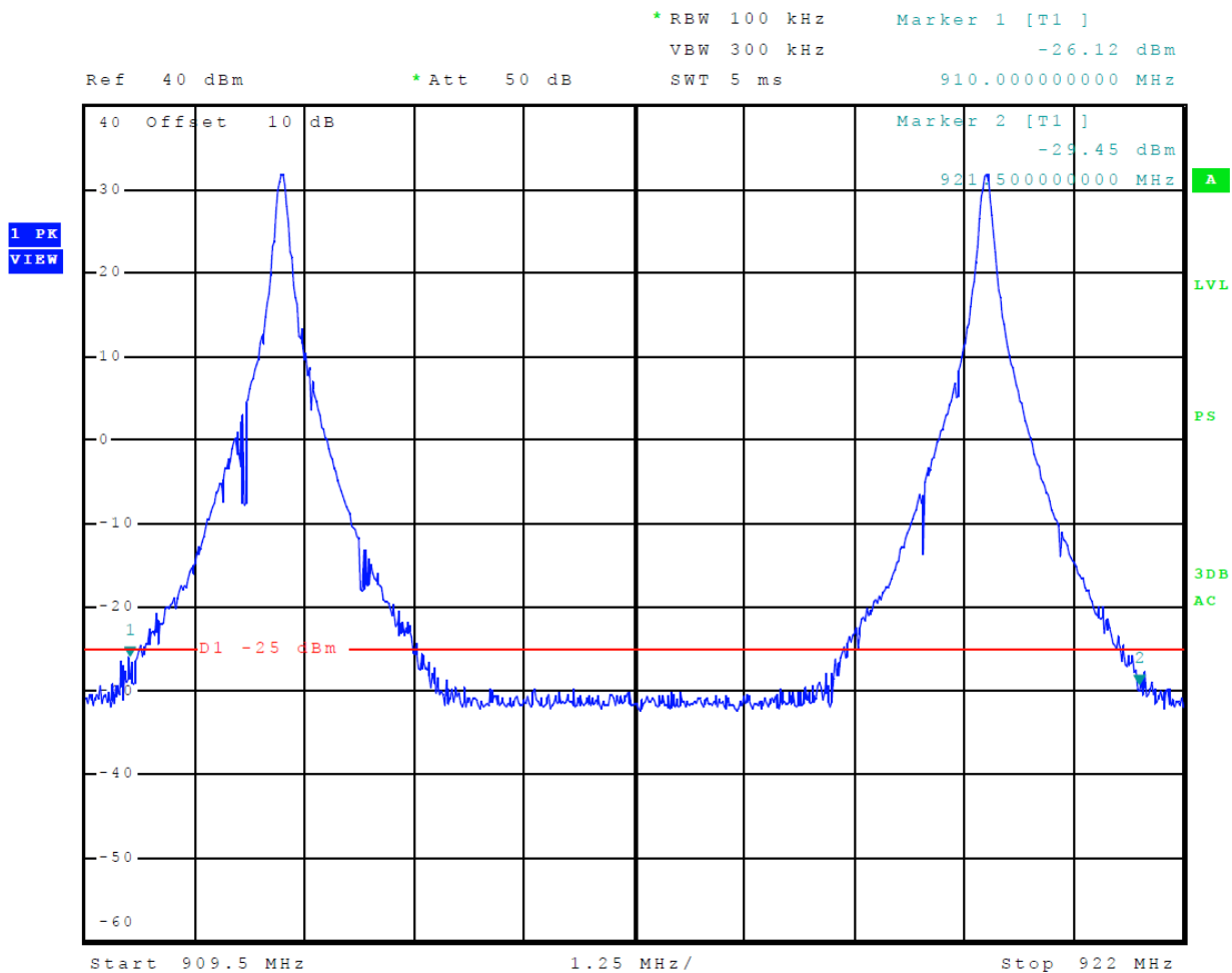
Figure 16 Emissions Mask IAG
