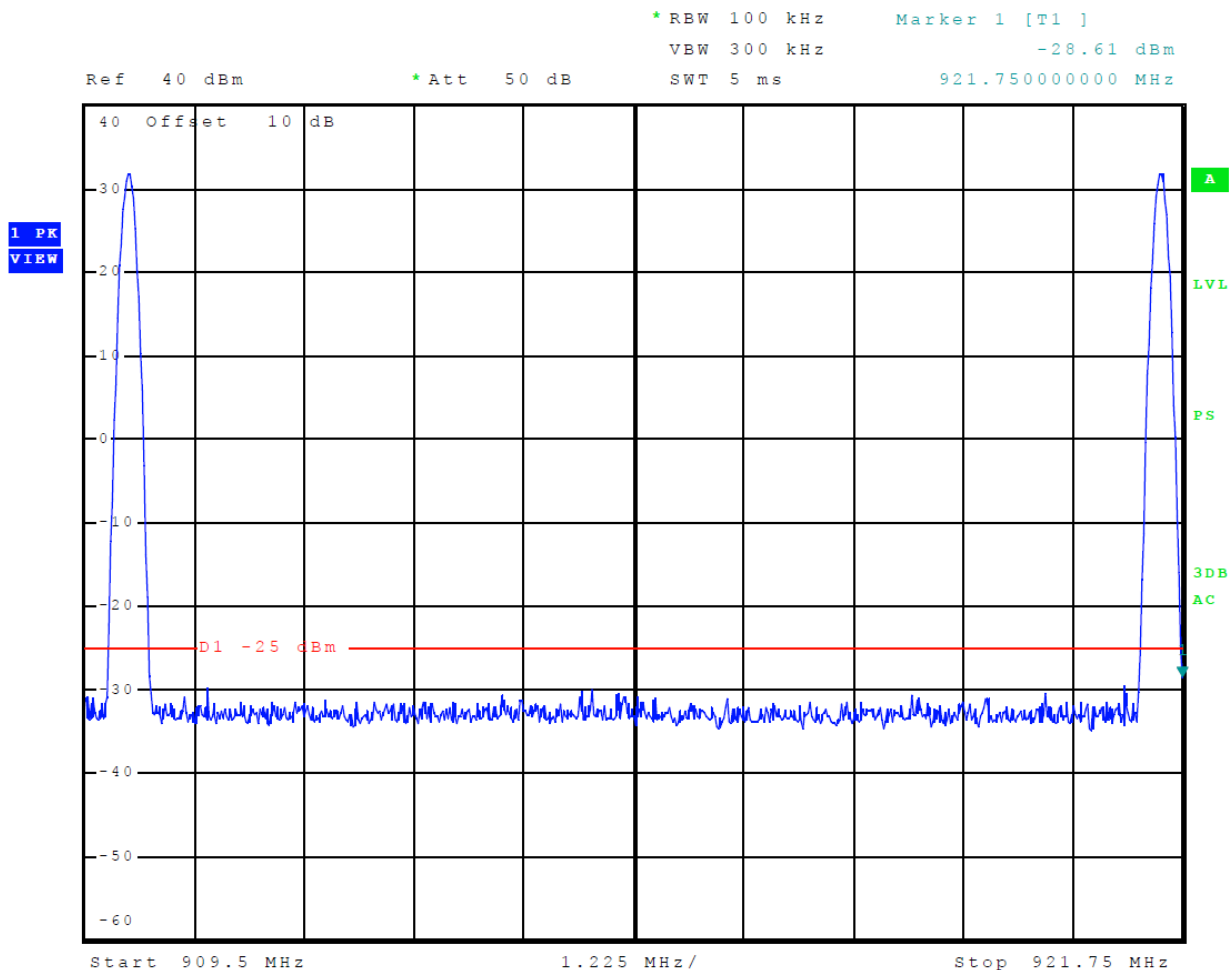
Figure 13 Emissions Mask ATA
