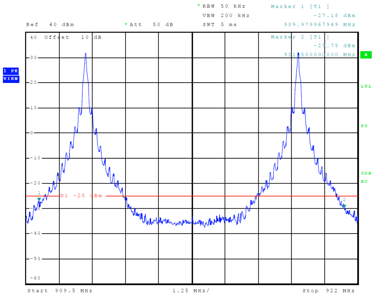
Figure 15 Emissions Mask SeGo
