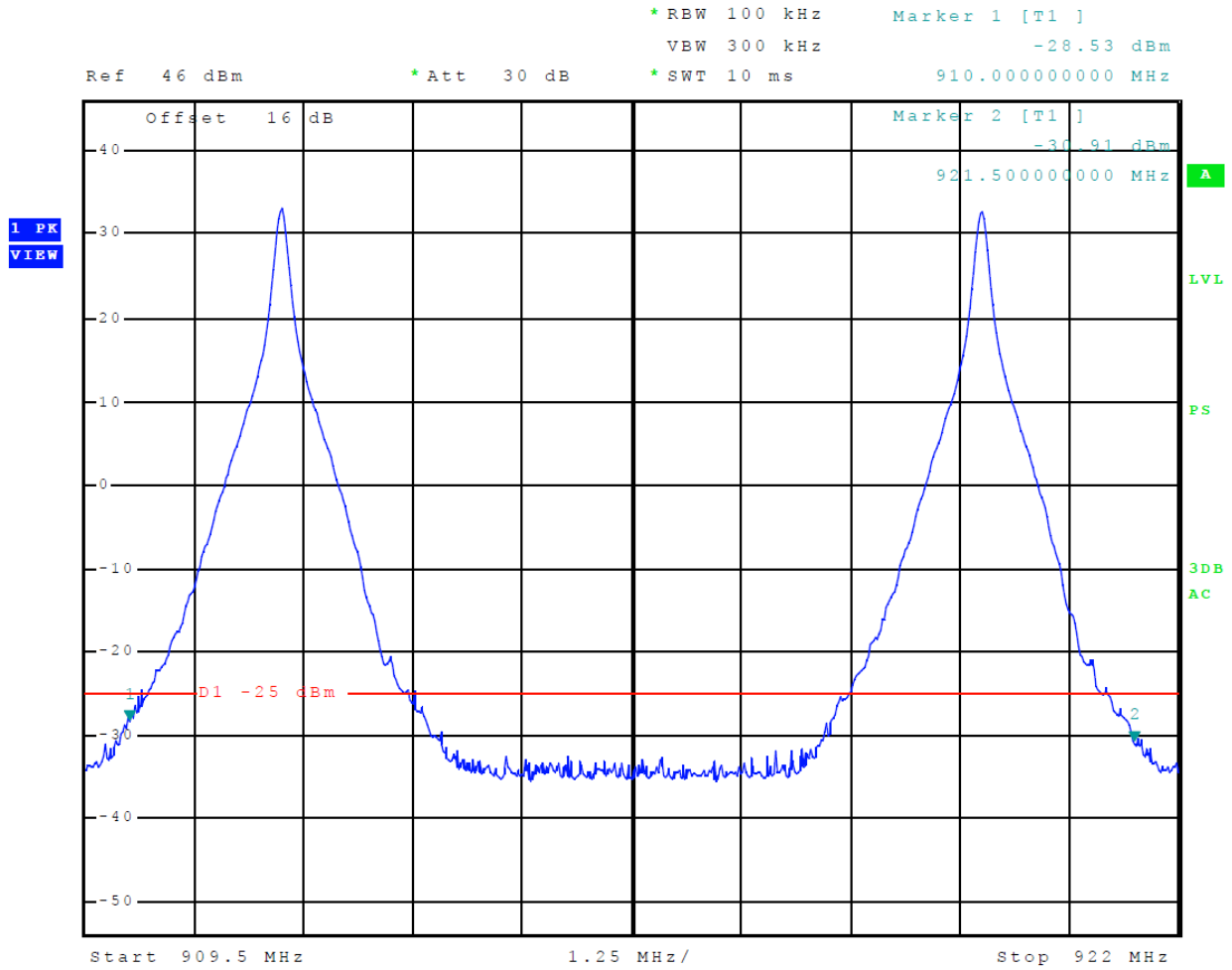
Figure 12 Emissions Mask eGo
