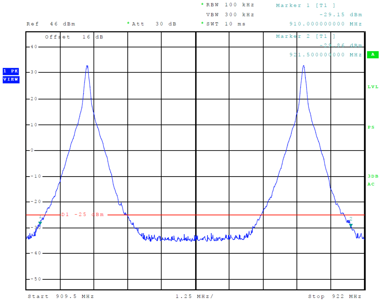
Figure 13 Emissions Mask SeGo
