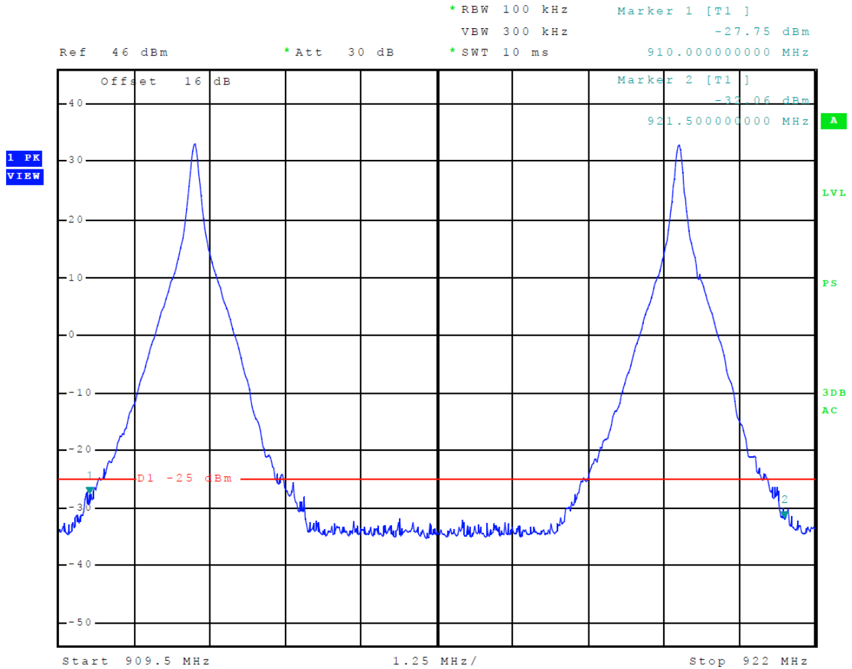
Figure 14 Emissions Mask IAG
