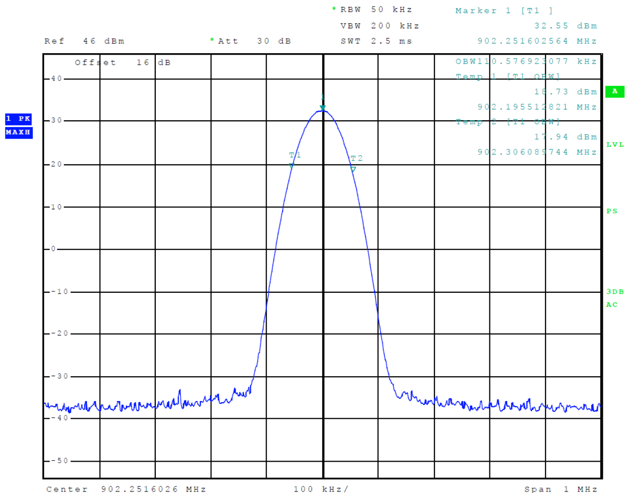
Figure 9 Occupied Bandwidth ATA
