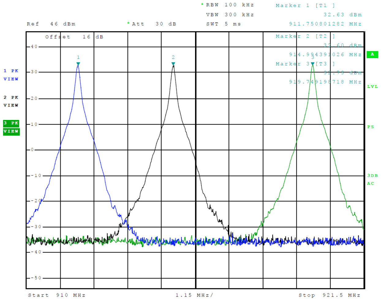
Figure 7 Transmitter Output Across Frequency Band EPC T1D
