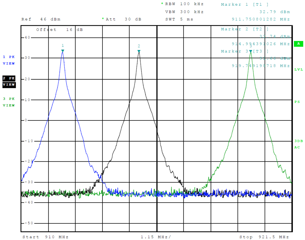
Figure 8 Transmitter Output Across Frequency Band EPC Sort
