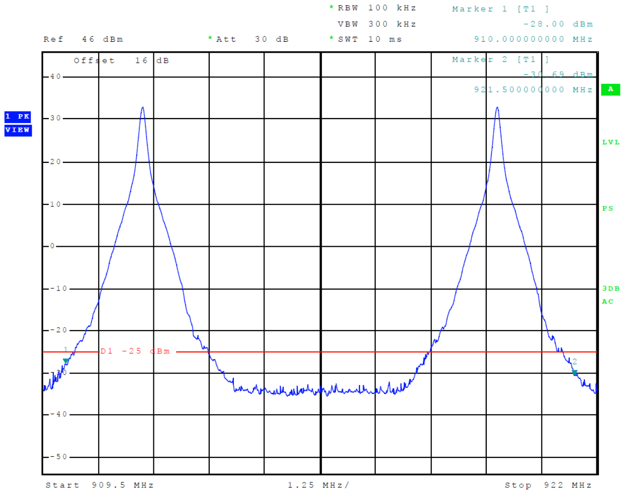
Figure 16 Emissions Mask EPC T1D
