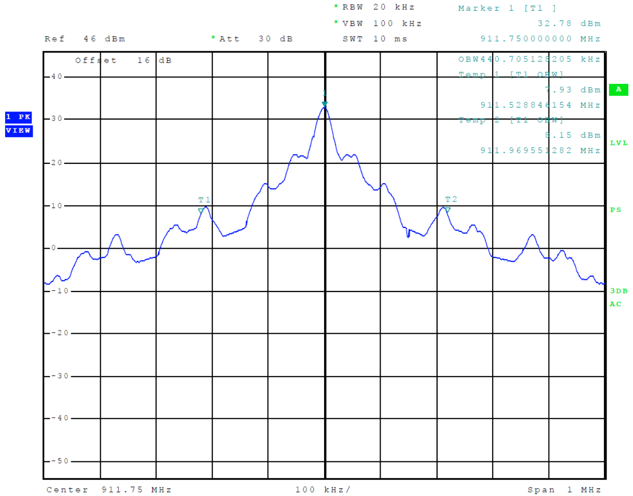
Figure 16 Occupied Bandwidth EPC Sort
