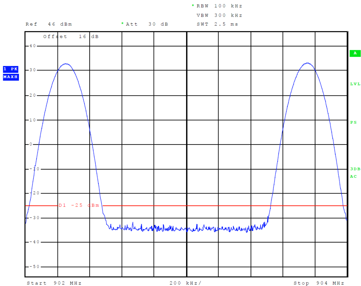
Figure 10 Emissions Mask ATA
