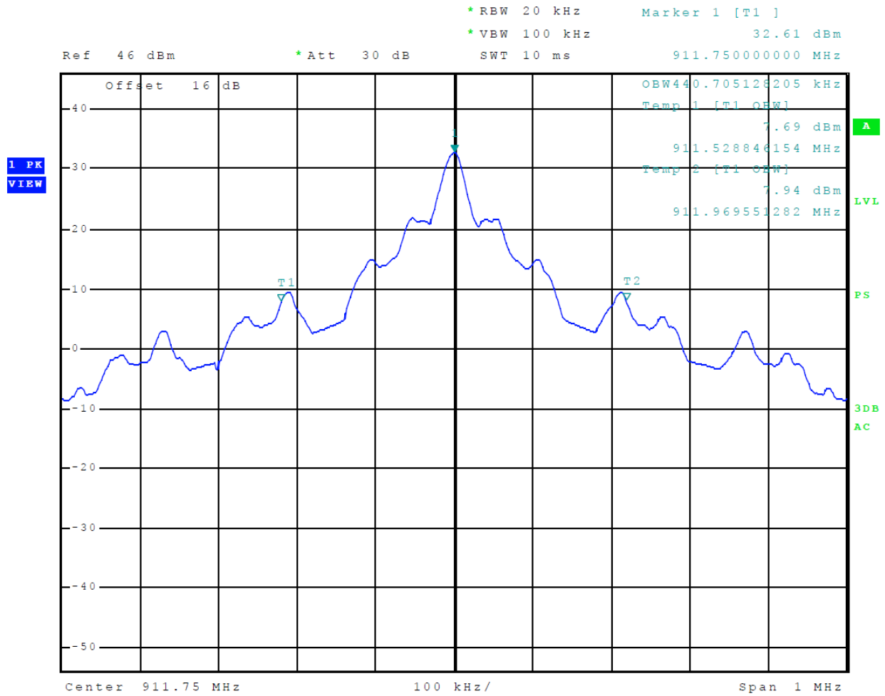
Figure 14 Occupied Bandwidth EPC
