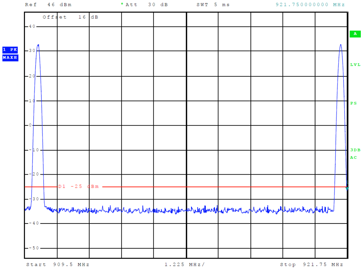
Figure 11 Emissions Mask ATA
