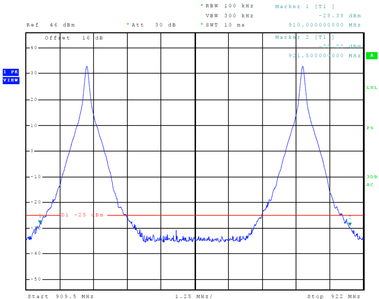
Figure 17 Emissions Mask EPC Sort
