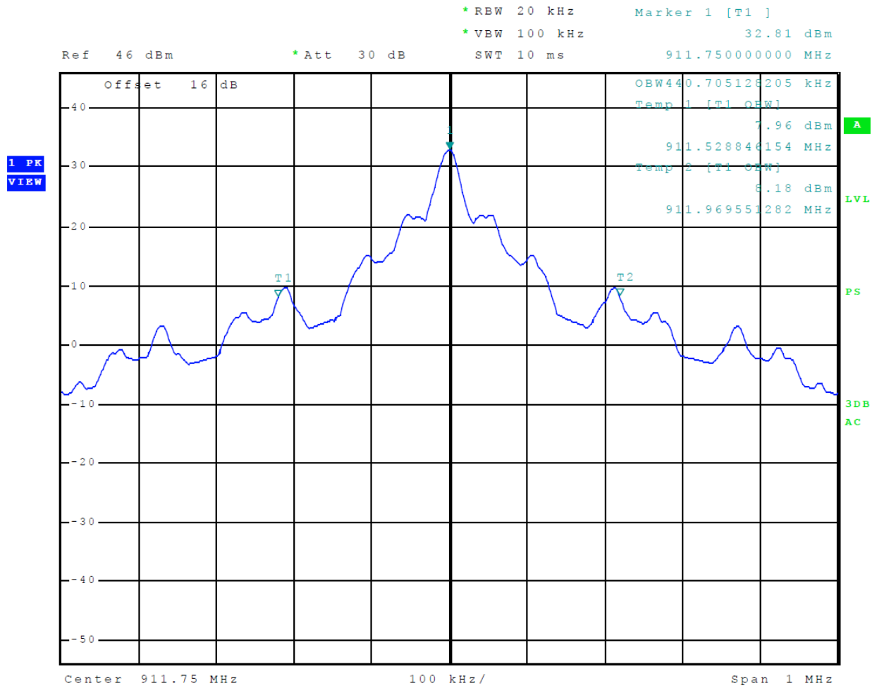
Figure 15 Occupied Bandwidth EPC T1D
