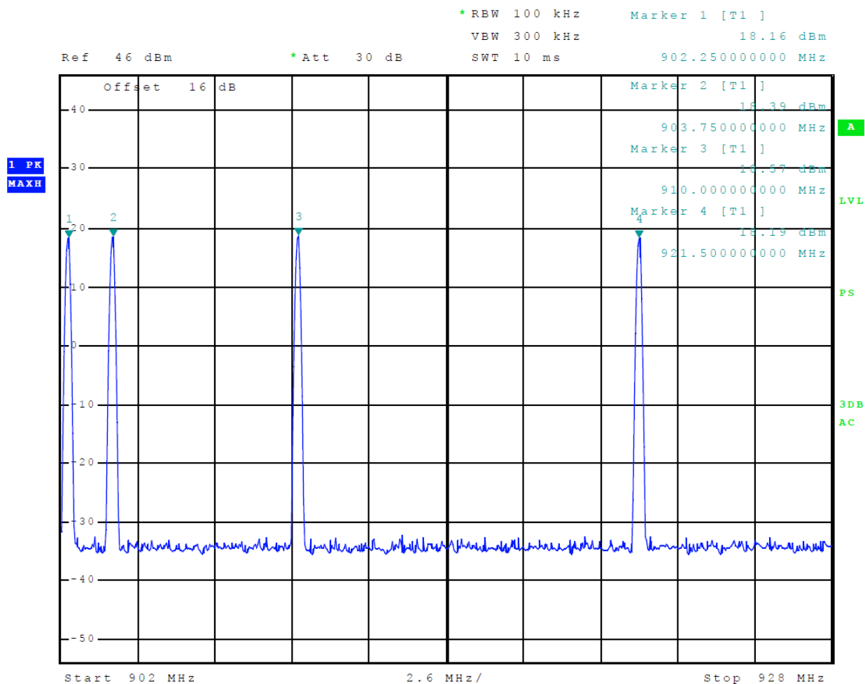
Figure 2 Transmitter Output Across Frequency Band ATA Lowest Power Level
