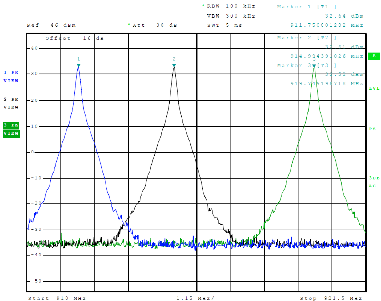
Figure 6 Transmitter Output Across Frequency Band EPC
