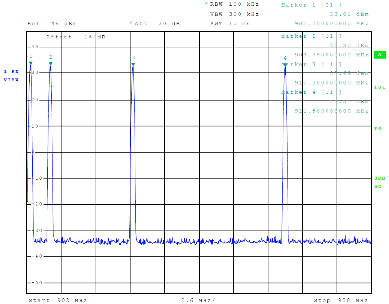
Figure 1 Transmitter Output Across Frequency Band ATA Highest Power Level
