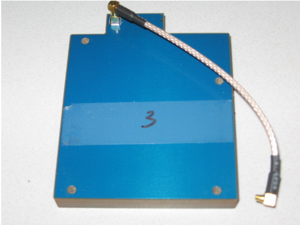
Authorized Patch Antenna (PN 07558-01) front
