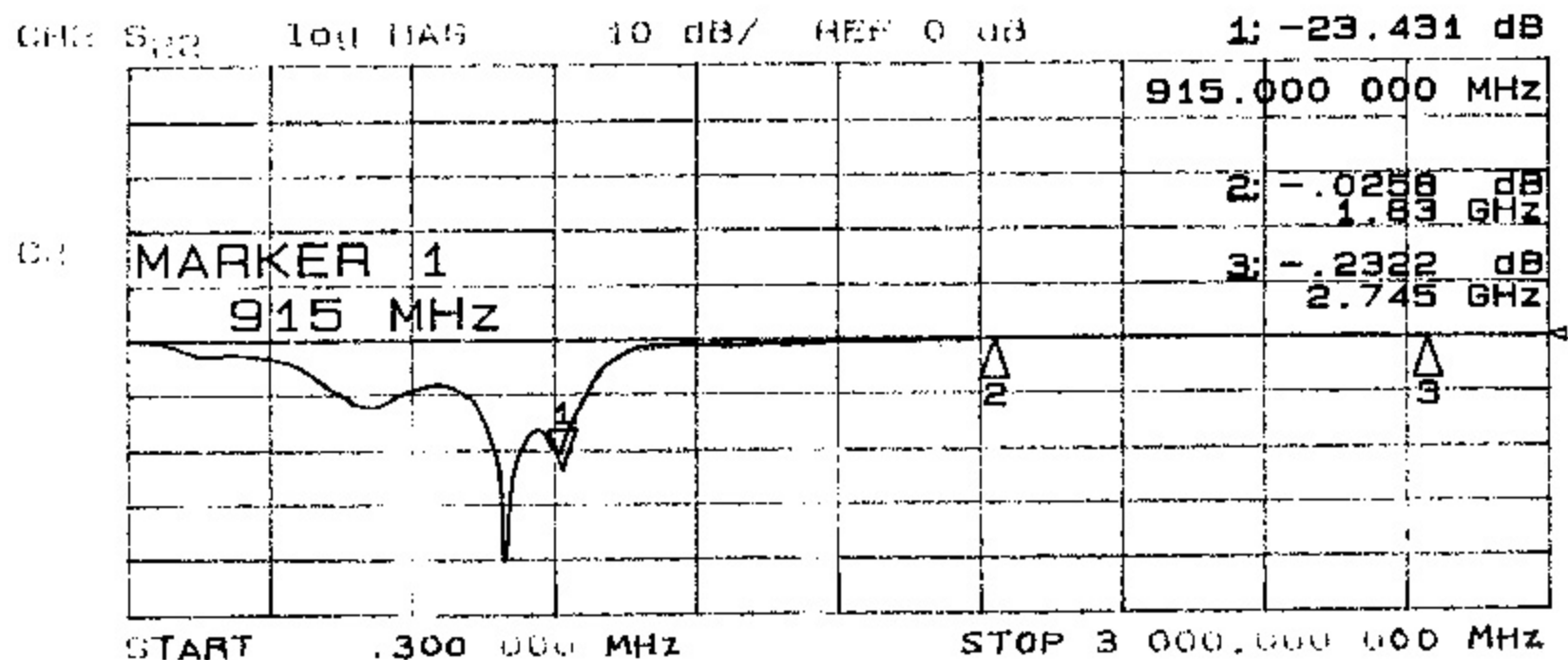
Figure 1. Measured Frequency Response of Transmitter Harmonic Filter
