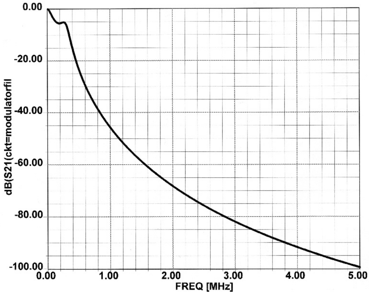
Figure 2. Predicted Frequency Response of Modulation Limiting Filter
