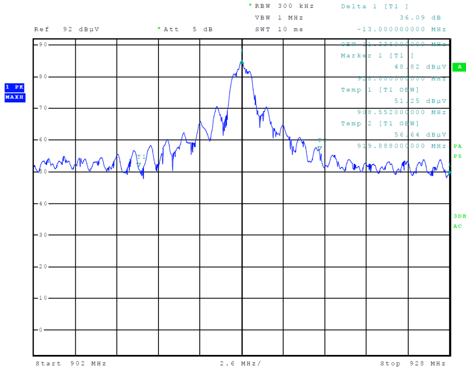
Figure 3 Occupied Bandwidth
