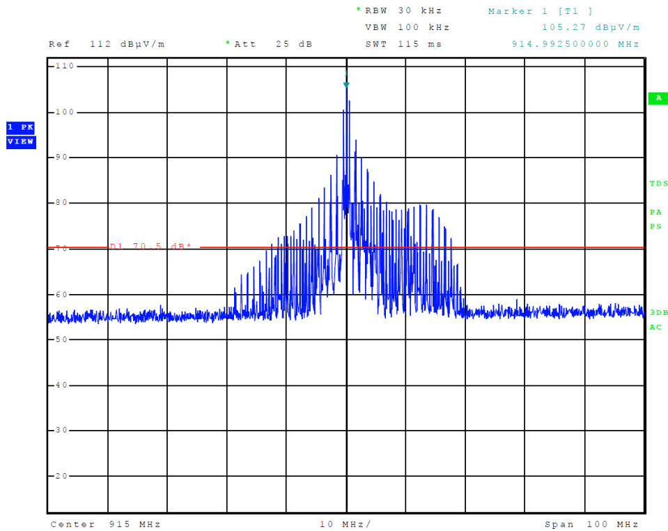
Figure 5 Emissions Mask High power
