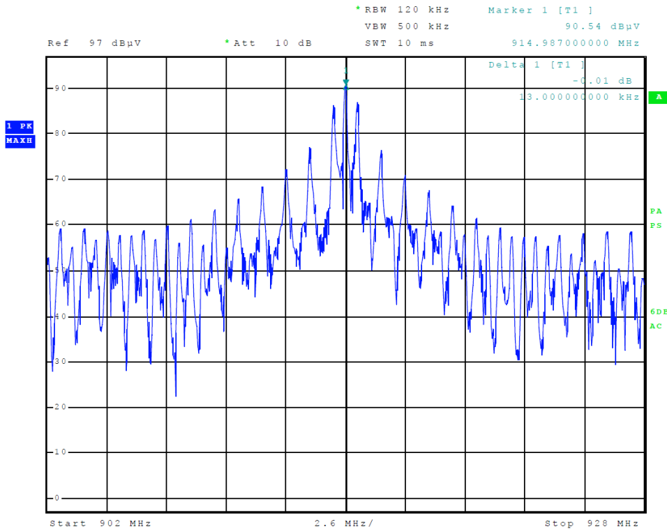
Figure 2 Transmitter Output across Frequency Band Low power mode
