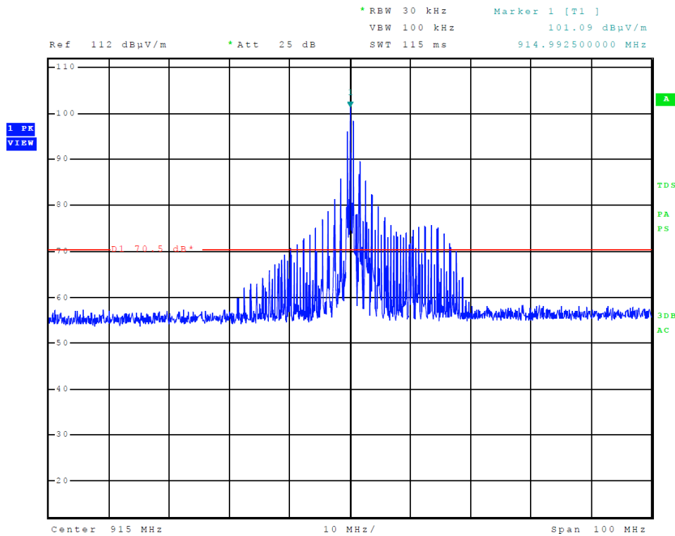
Figure 4 Emissions Mask Low power
