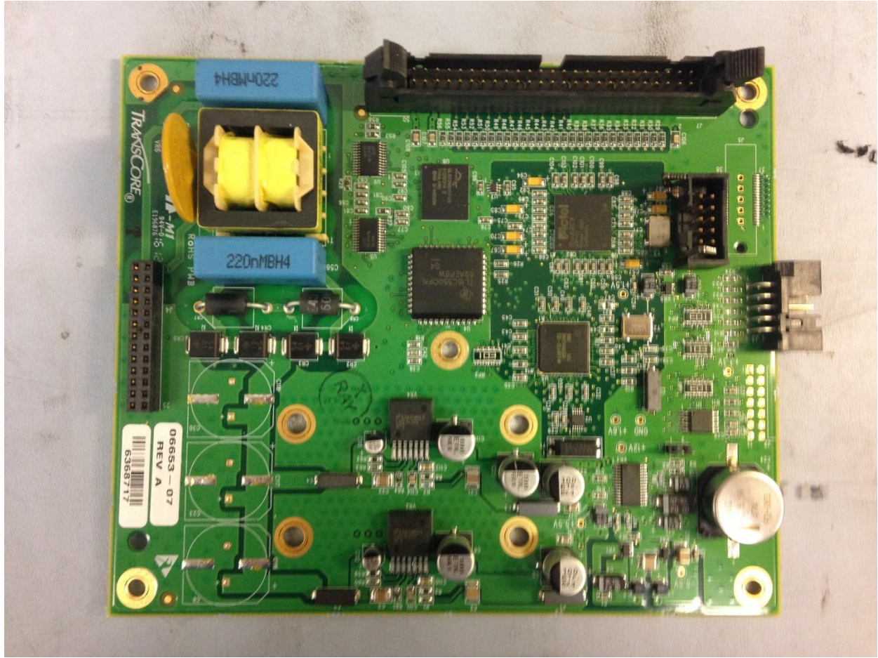
Processor Board Front
