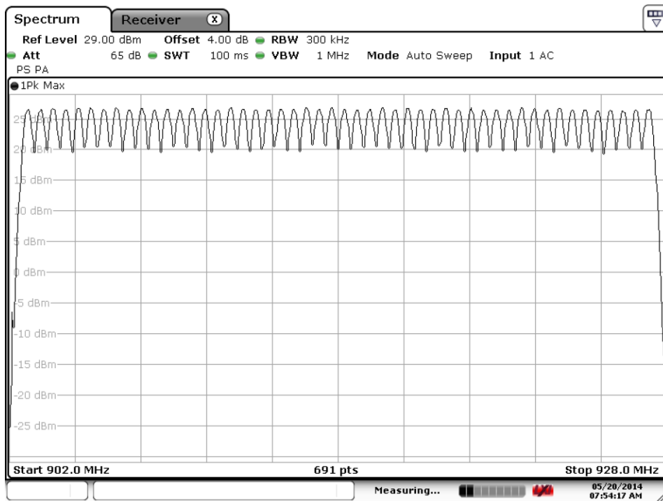
Figure 3 Plot of Transmitter Emissions in Operational Frequency (number of Hops)
