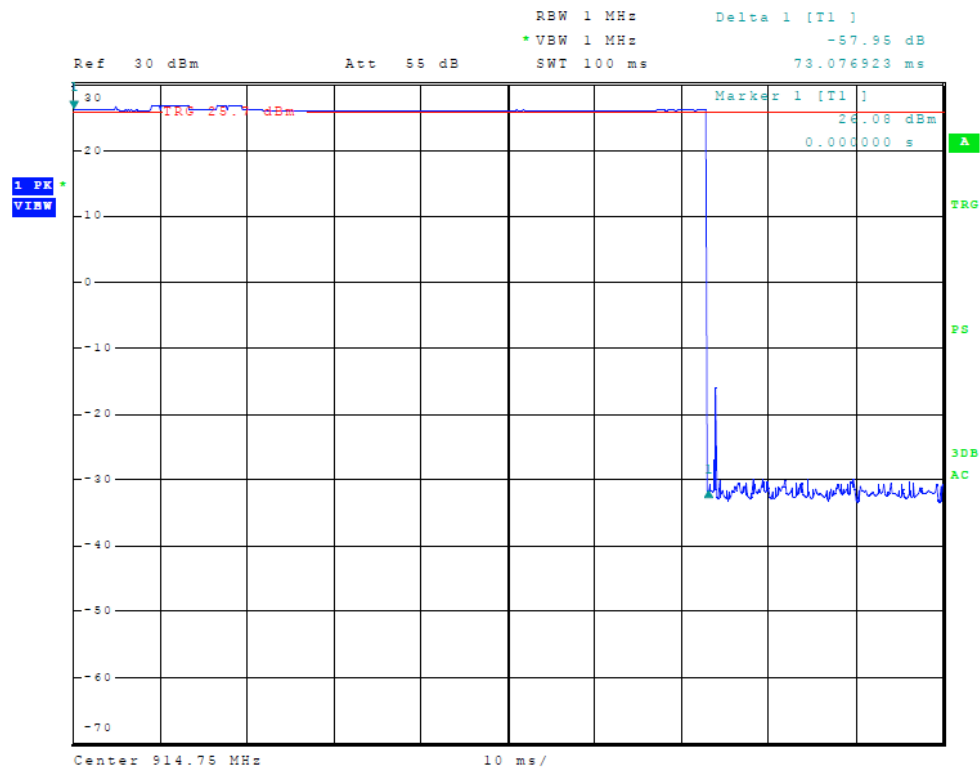
Figure 7 Plot of Transmitter Dwell Time on Channel
