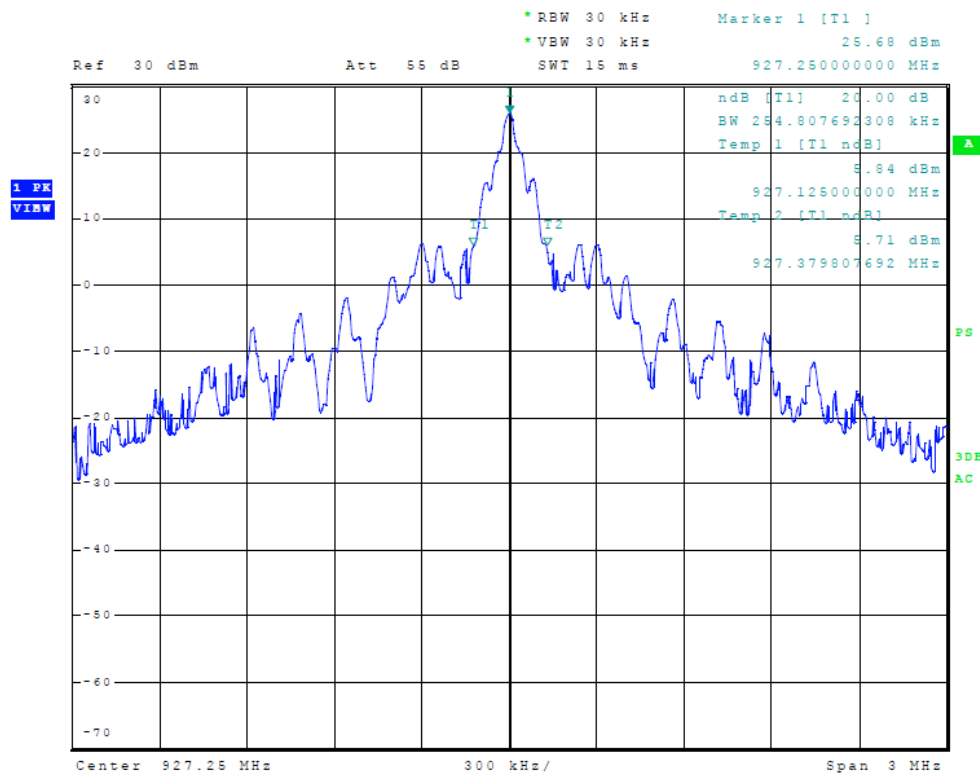
Figure 6 Plot of Transmitter Occupied Bandwidth (20-dB)
