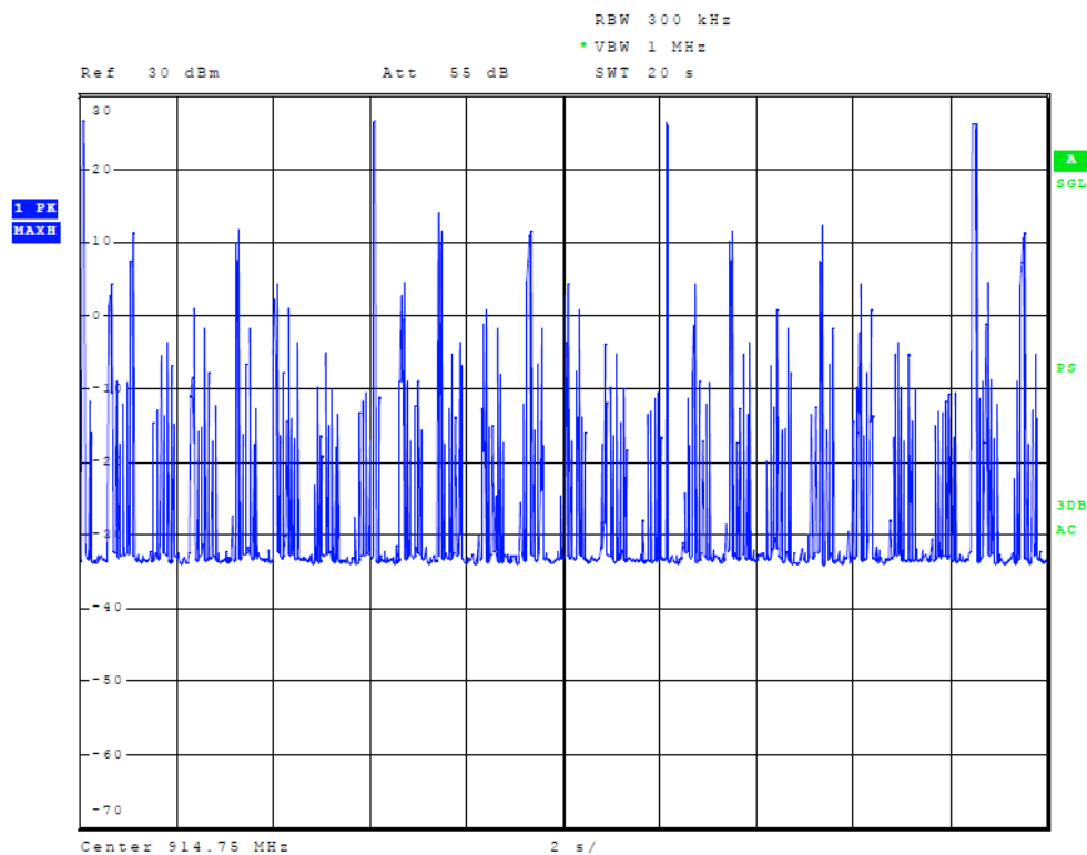
Figure 8 Plot of Number of Times Transmitter on Channel
