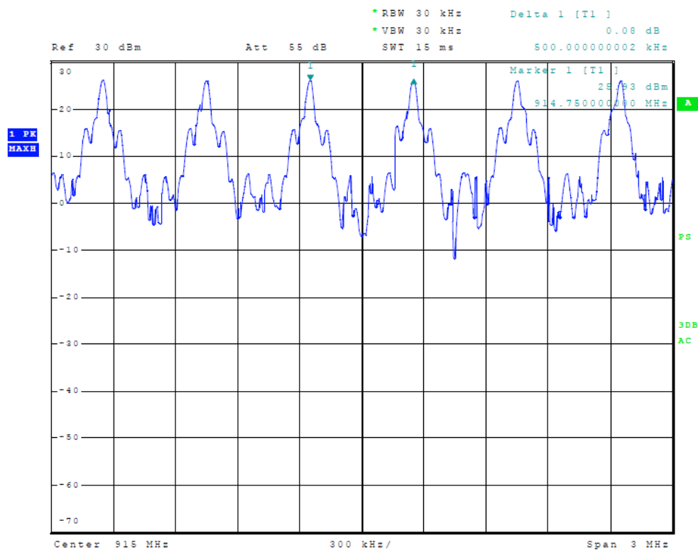
Figure 4 Plot of Transmitter Channel Spacing
