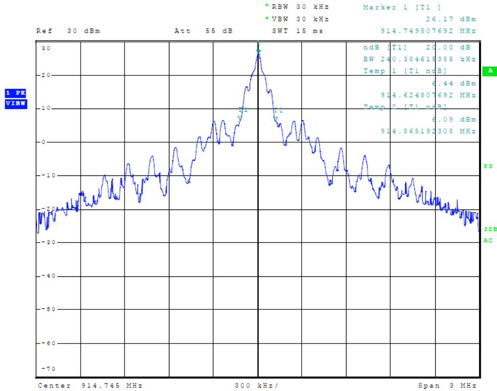
Figure 5 Plot of Transmitter Occupied Bandwidth (20-dB)
