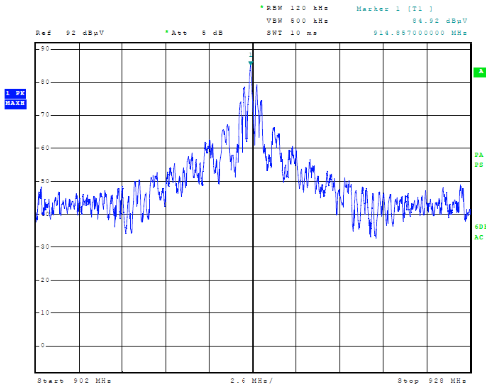
Figure 1 Power output
