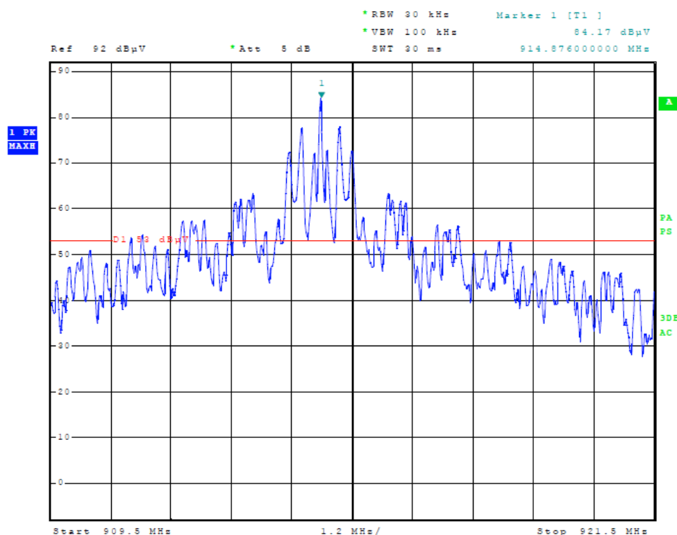
Figure 3 Emissions Mask
