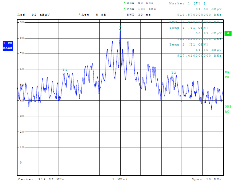
Figure 2 Occupied Bandwidth
