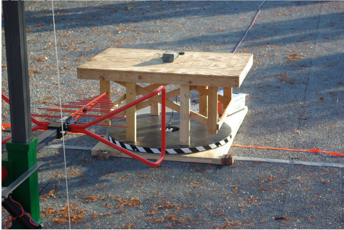
Equipment placed on OATS during testing
