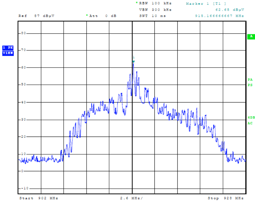
Figure Six Plot of in Frequency Band Emissions
