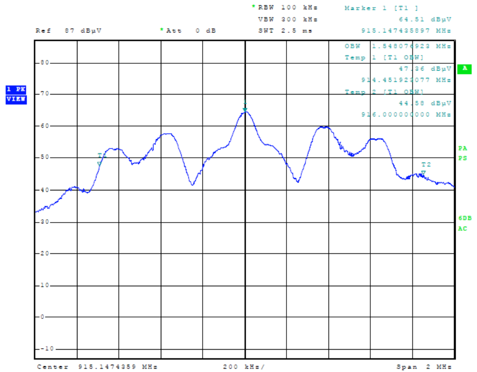
Figure Seven Plot of Occupied Bandwidth
