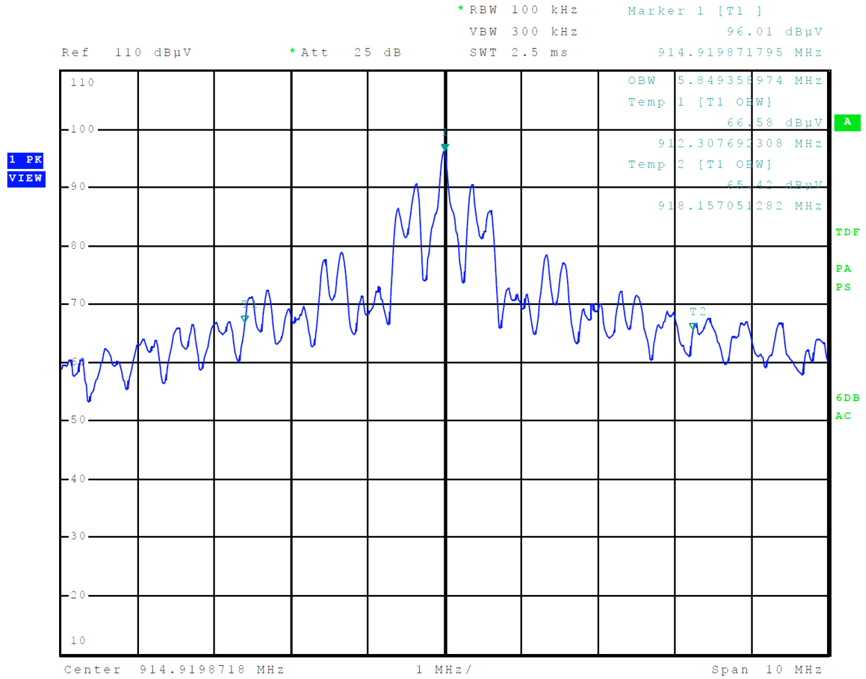
Figure 2 Occupied Bandwidth
