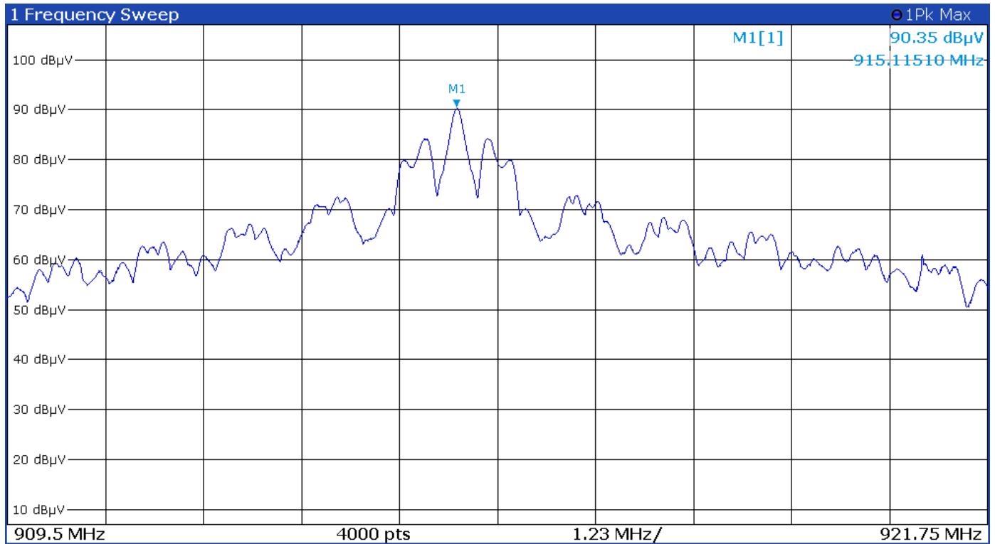
Figure 1 Transmitter Output Across Frequency Band
