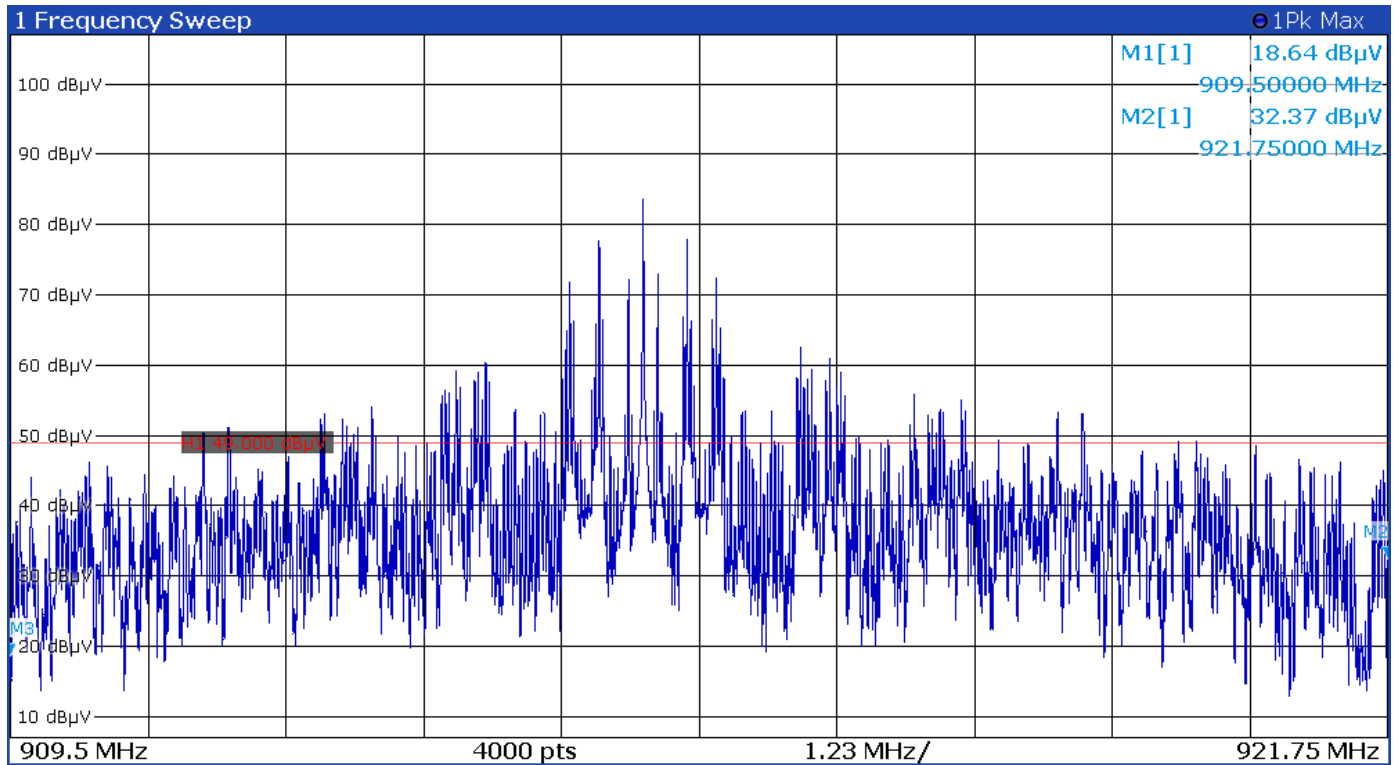
Figure 3 Emissions Mask
