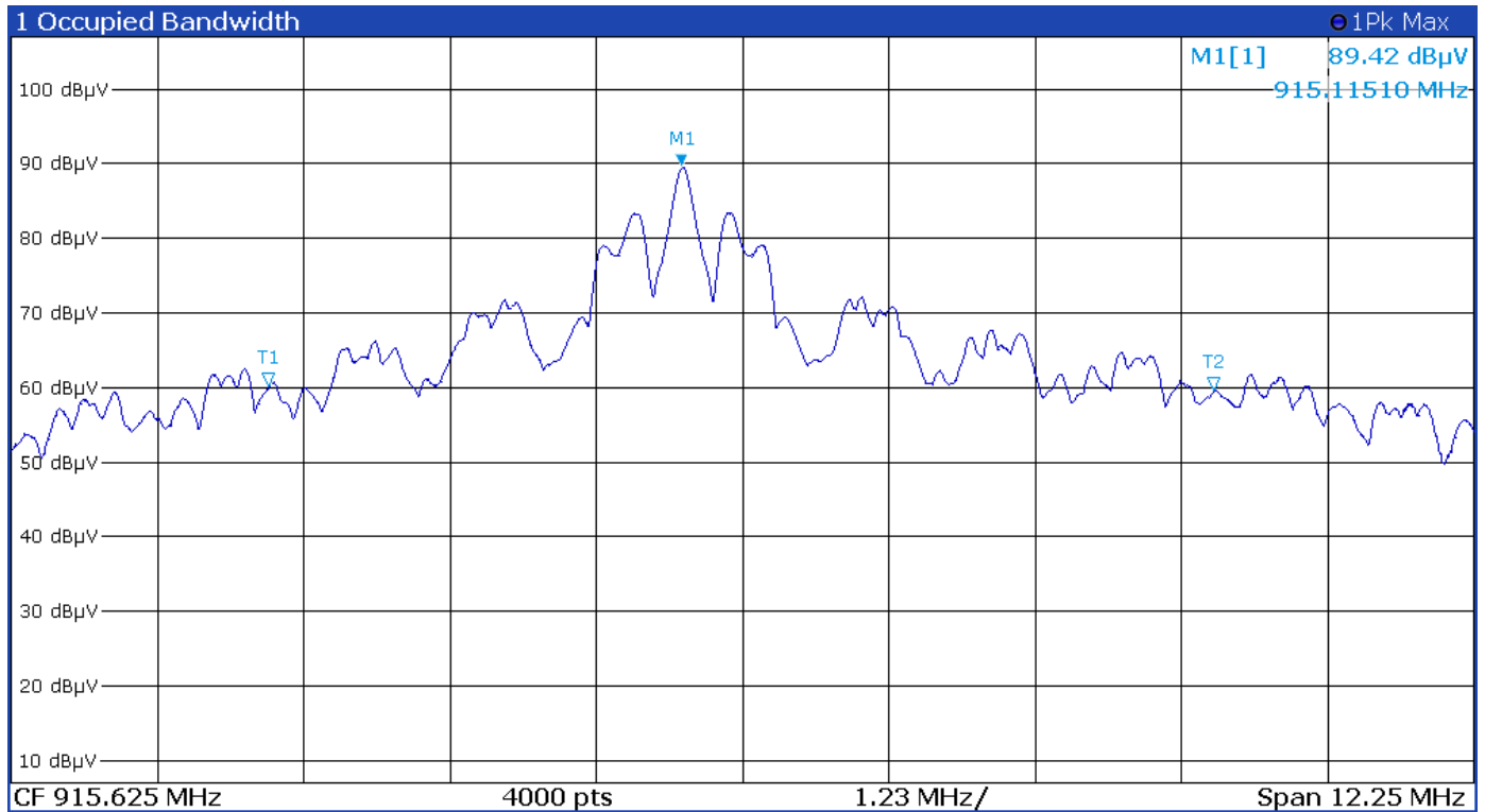
Figure 2 Occupied Bandwidth
