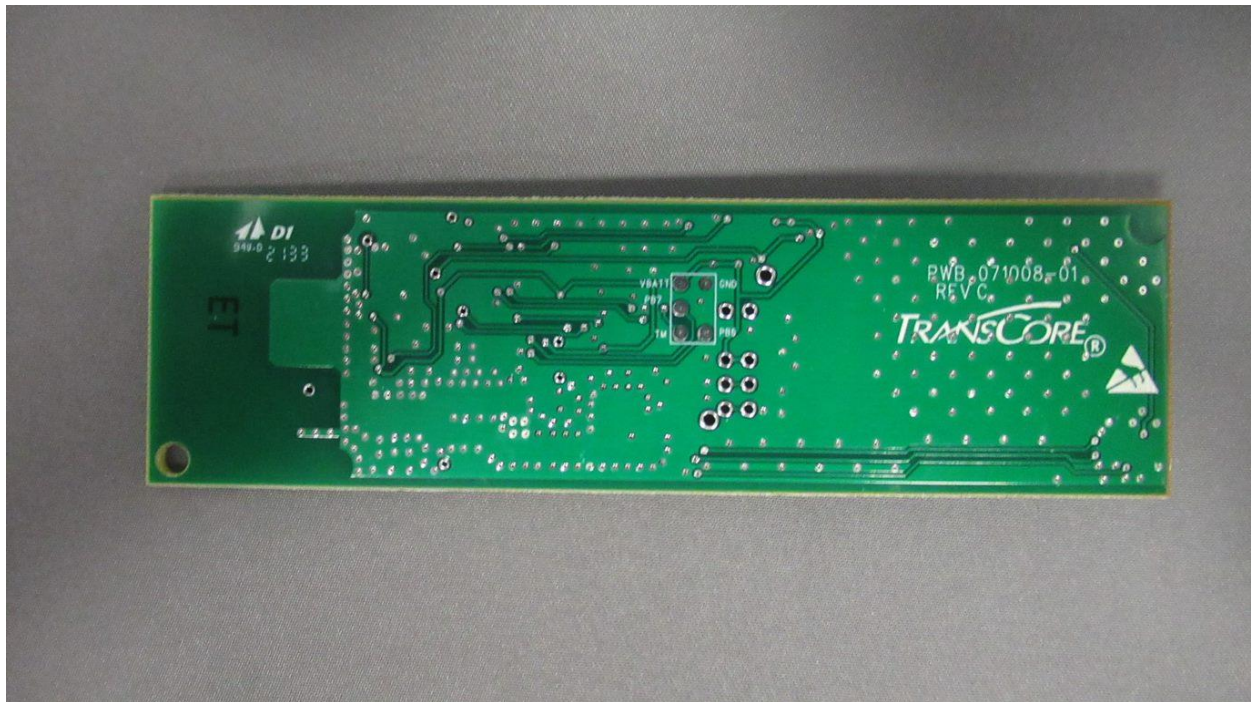
Transmitter PCB Back Side
