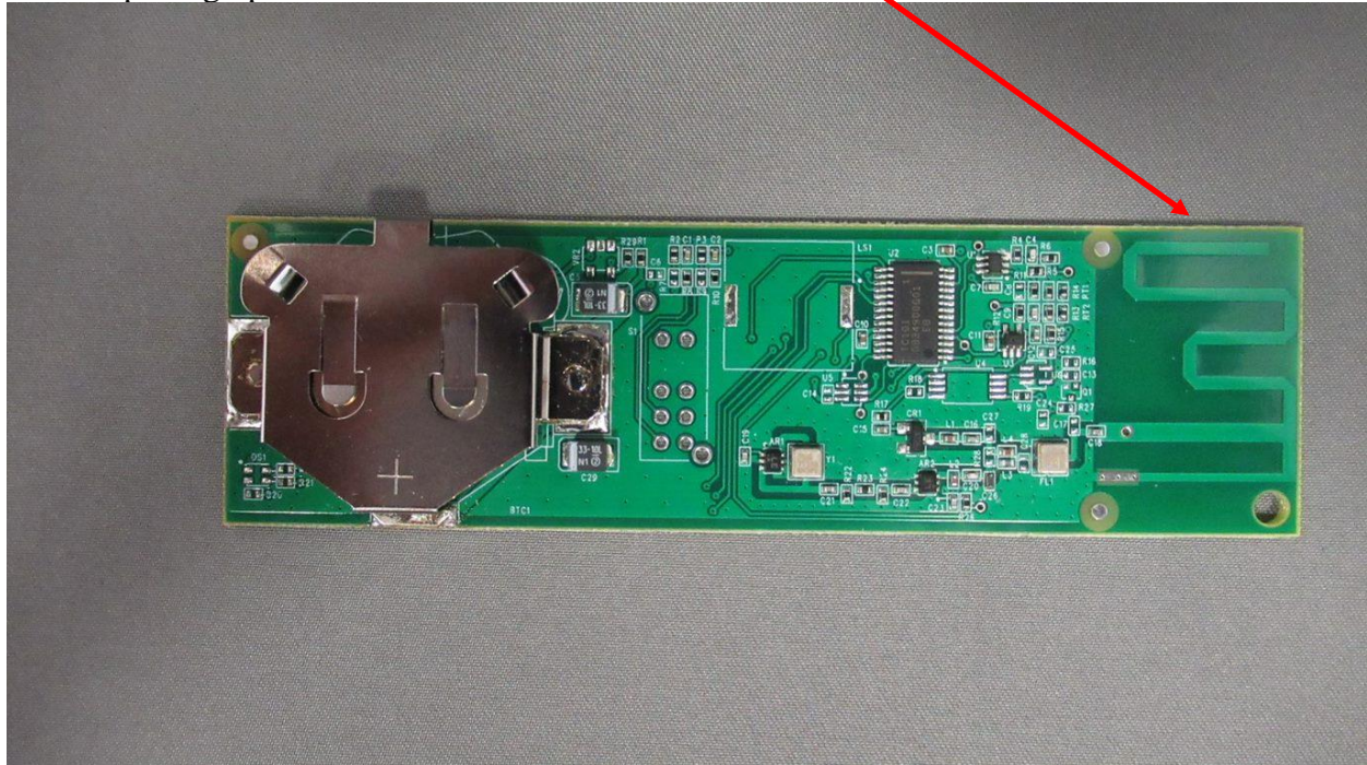
Internal photographs Transmitter PCB Front Side Antenna
