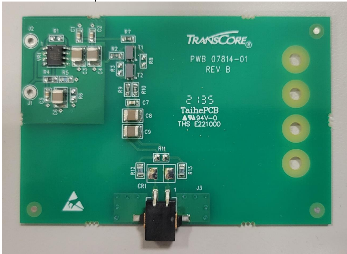
Power interface PCB Back
