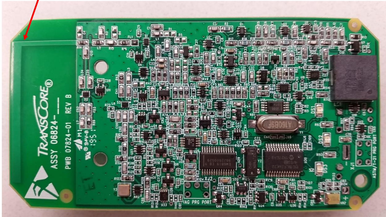
Internal photographs Transmitter PCB Front Side Antenna
