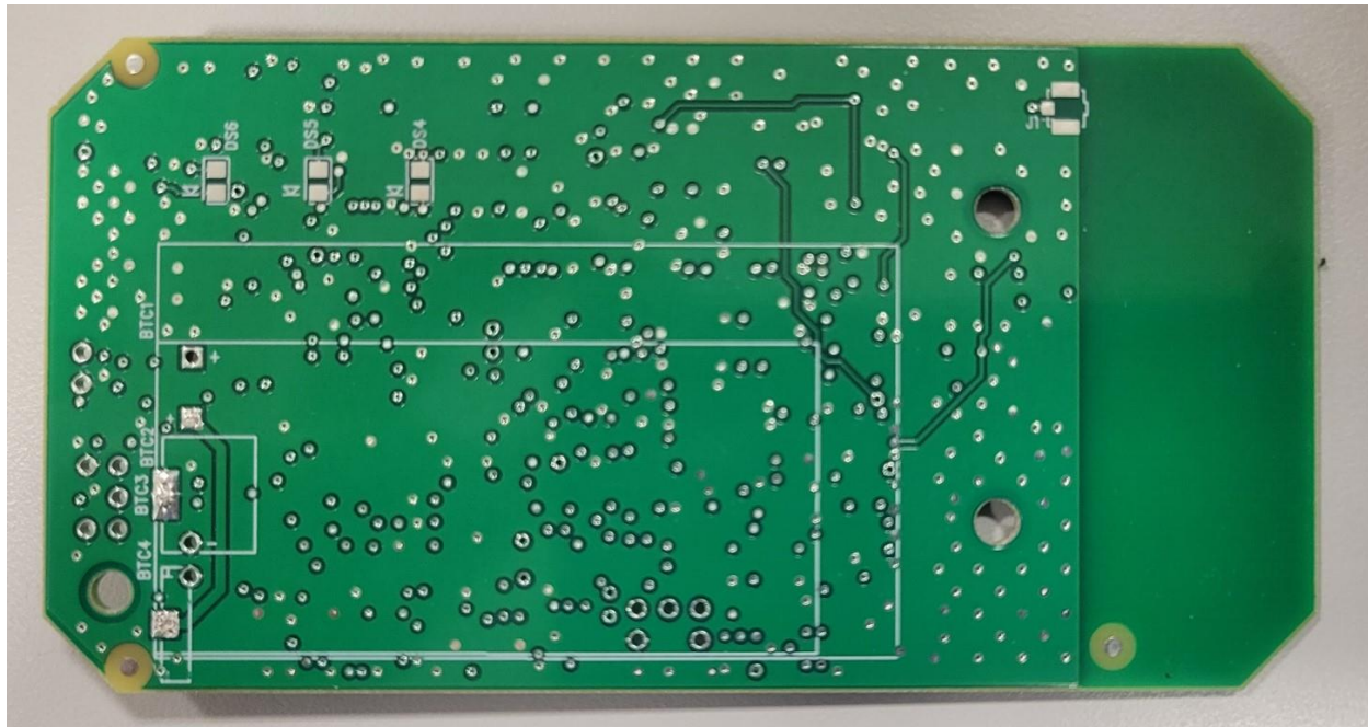
Transmitter PCB Back Side
