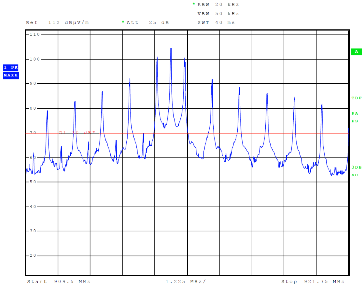
Figure 6 Emissions Mask IAG
