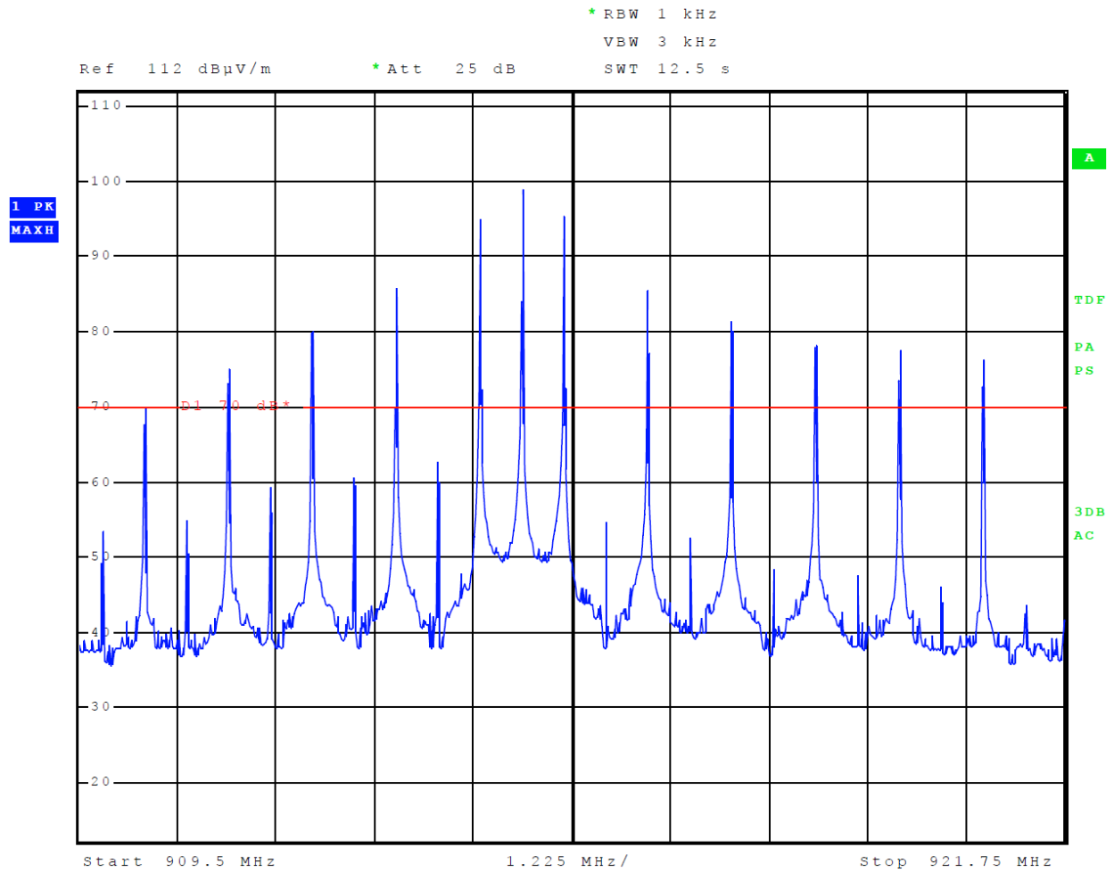
Figure 5 Emissions Mask ASTM
