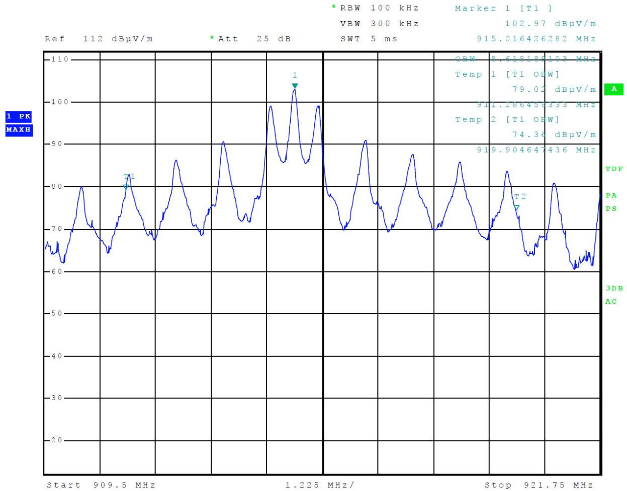
Figure 3 Occupied Bandwidth (ASTM)
