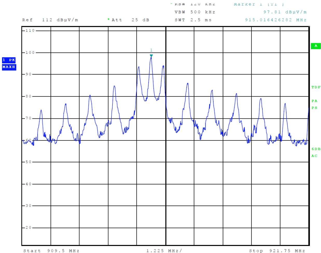
Figure 2 Transmitter Output Across Frequency Band (IAG)
