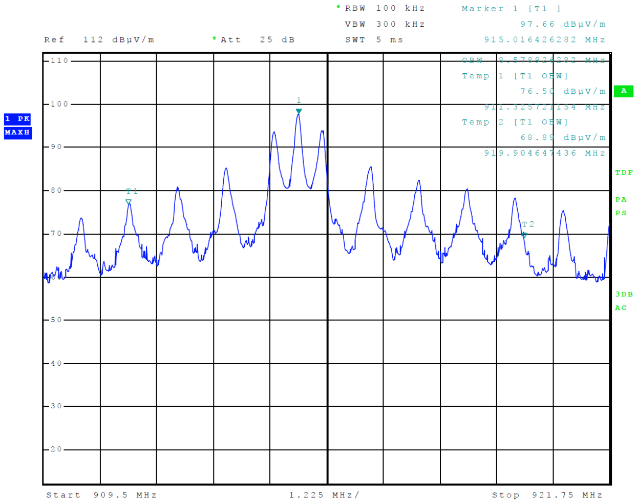
Figure 4 Occupied Bandwidth (IAG)
