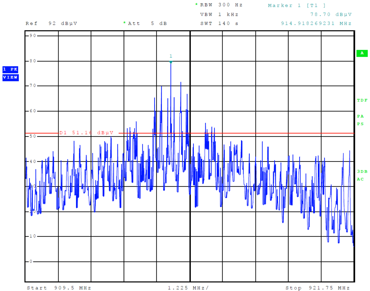
Figure 5 IAG Emissions Mask
