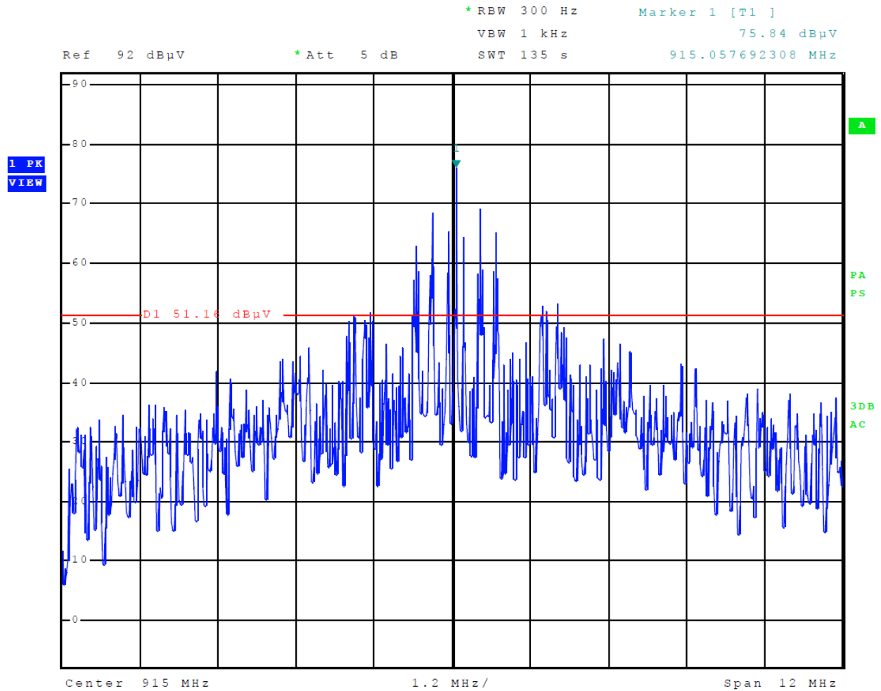
Figure 6 ASTM Emissions Mask
