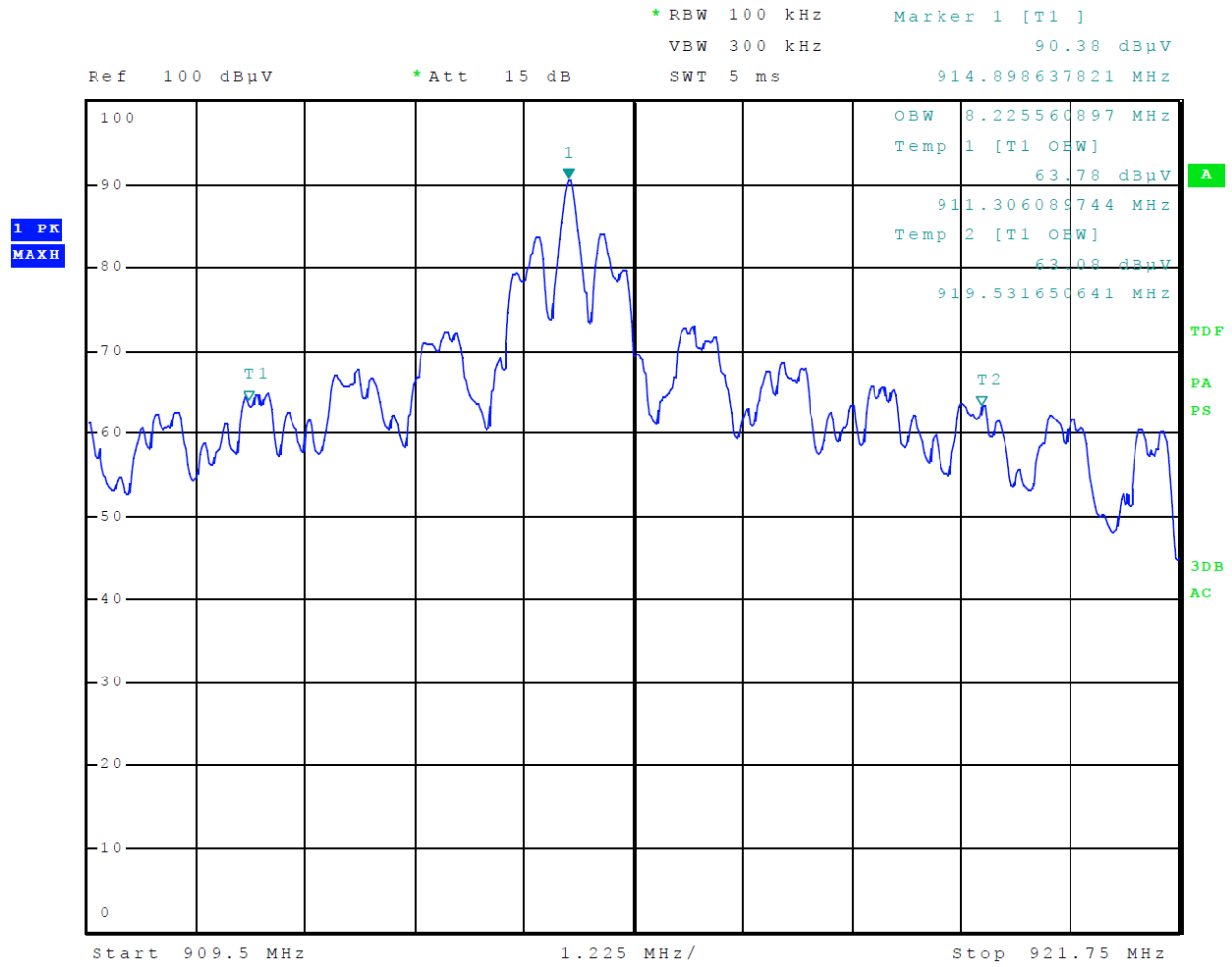
Figure 4 ASTM Occupied Bandwidth
