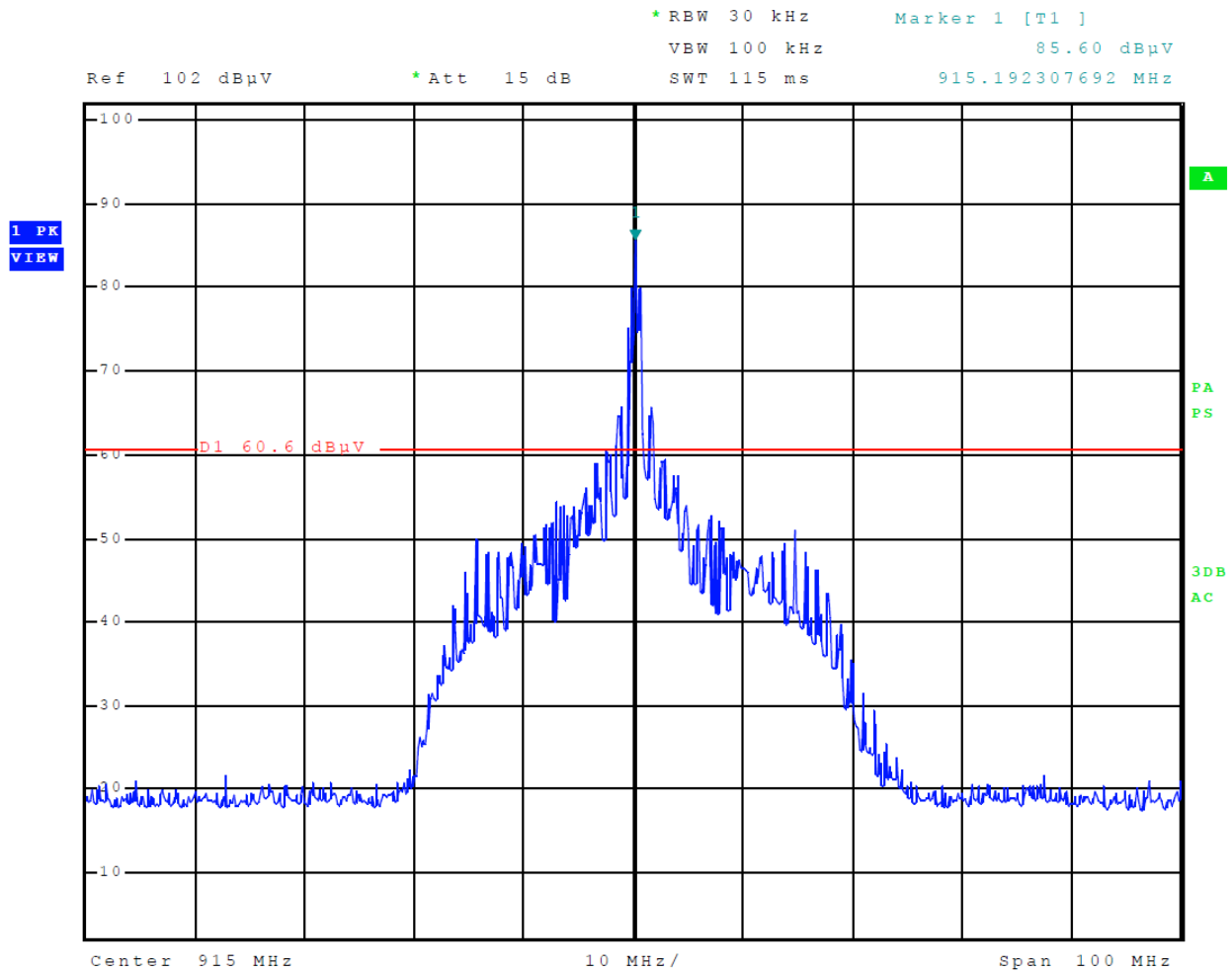
Figure 4 Emissions Mask
