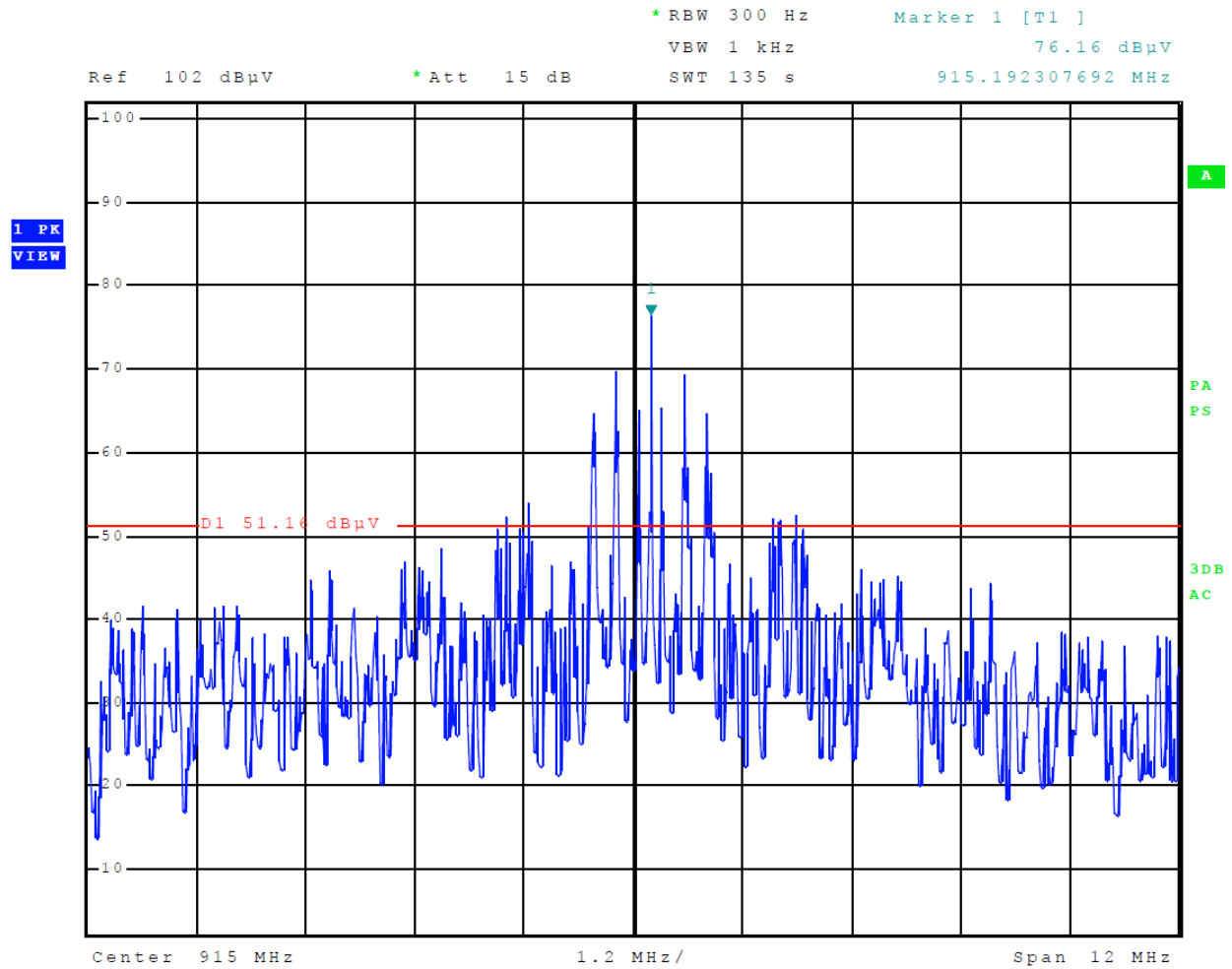
Figure 3 Emissions Mask
