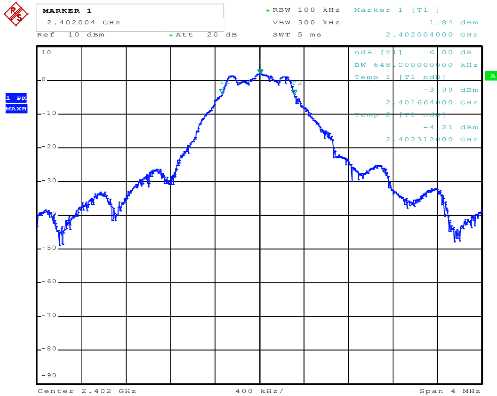
6dB bandwidth – Channel 2402 MHz
