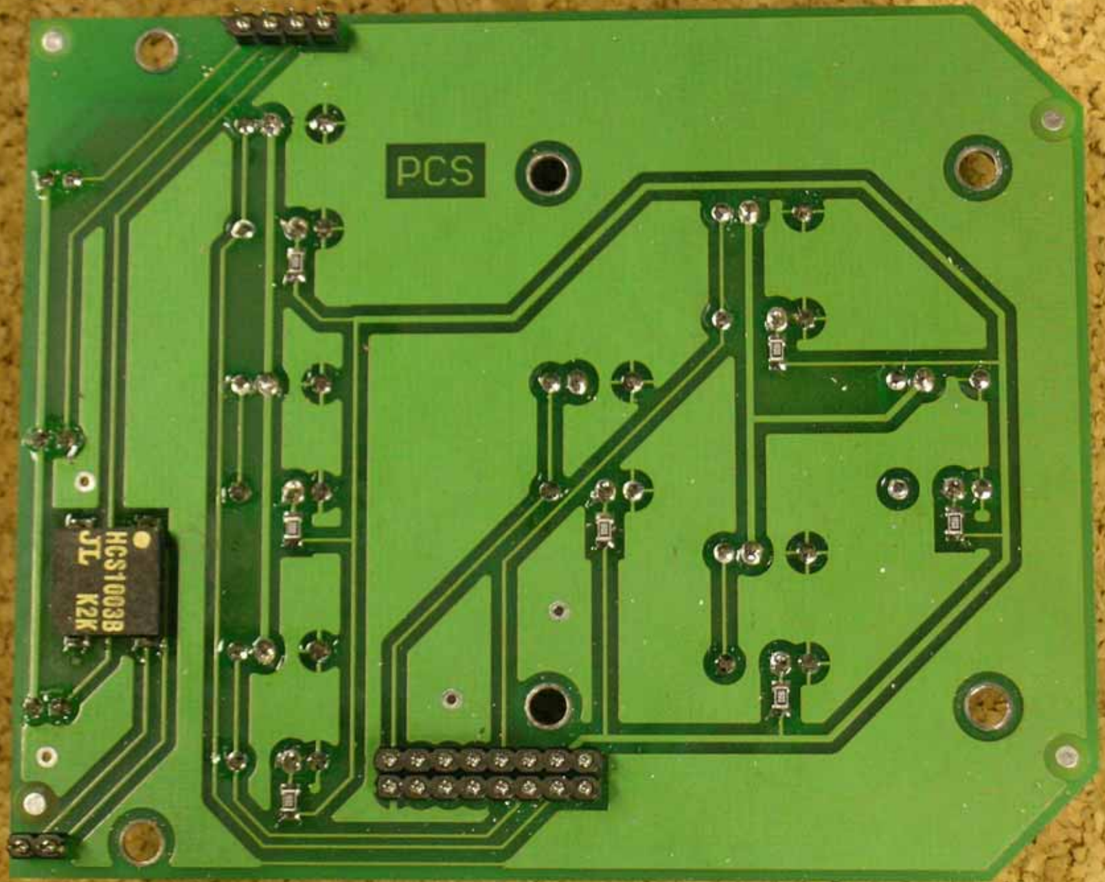
PCB (bottom)
