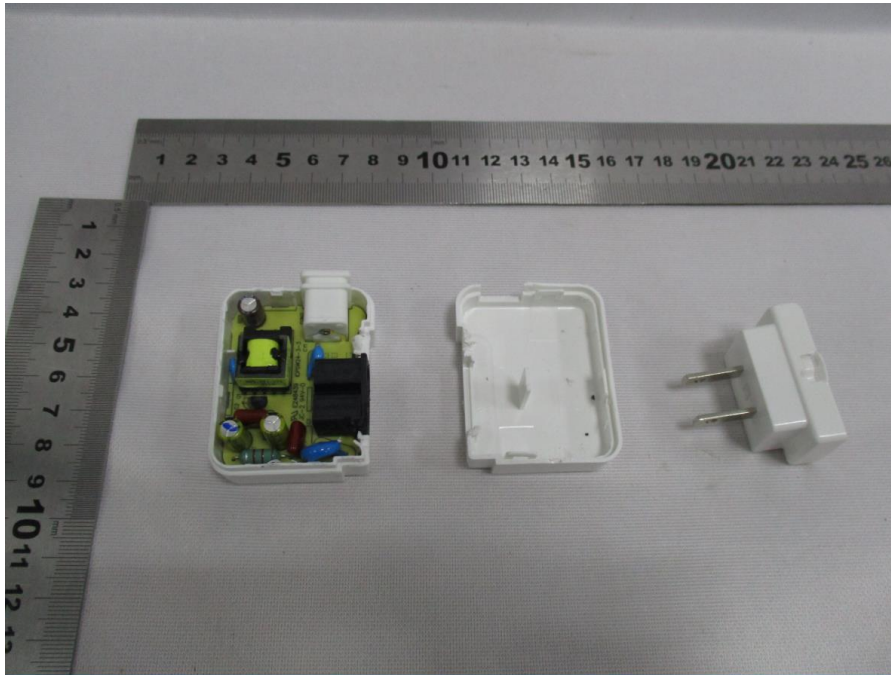
Open view of LED driver
