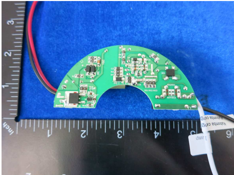
Rear of PCB
