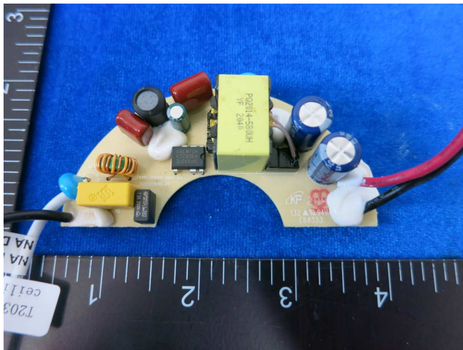
Front of LED Driver PCB
