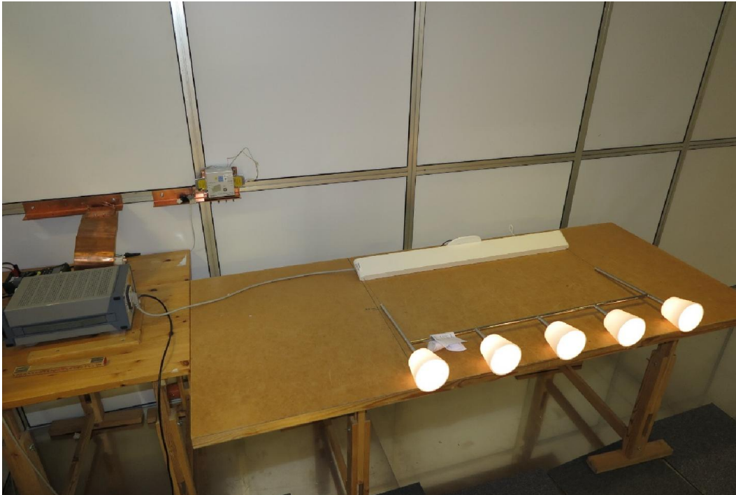
Test setup for conducted emission 150 kHz – 30 MHz
