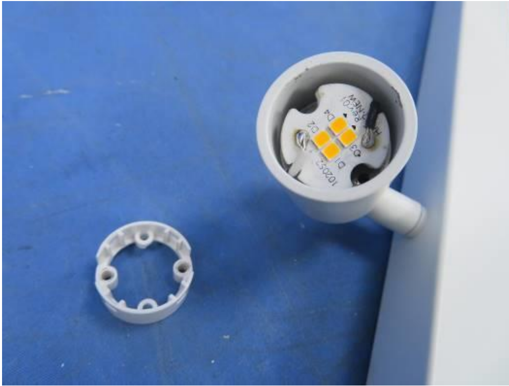
Photo 12 - Internal view
